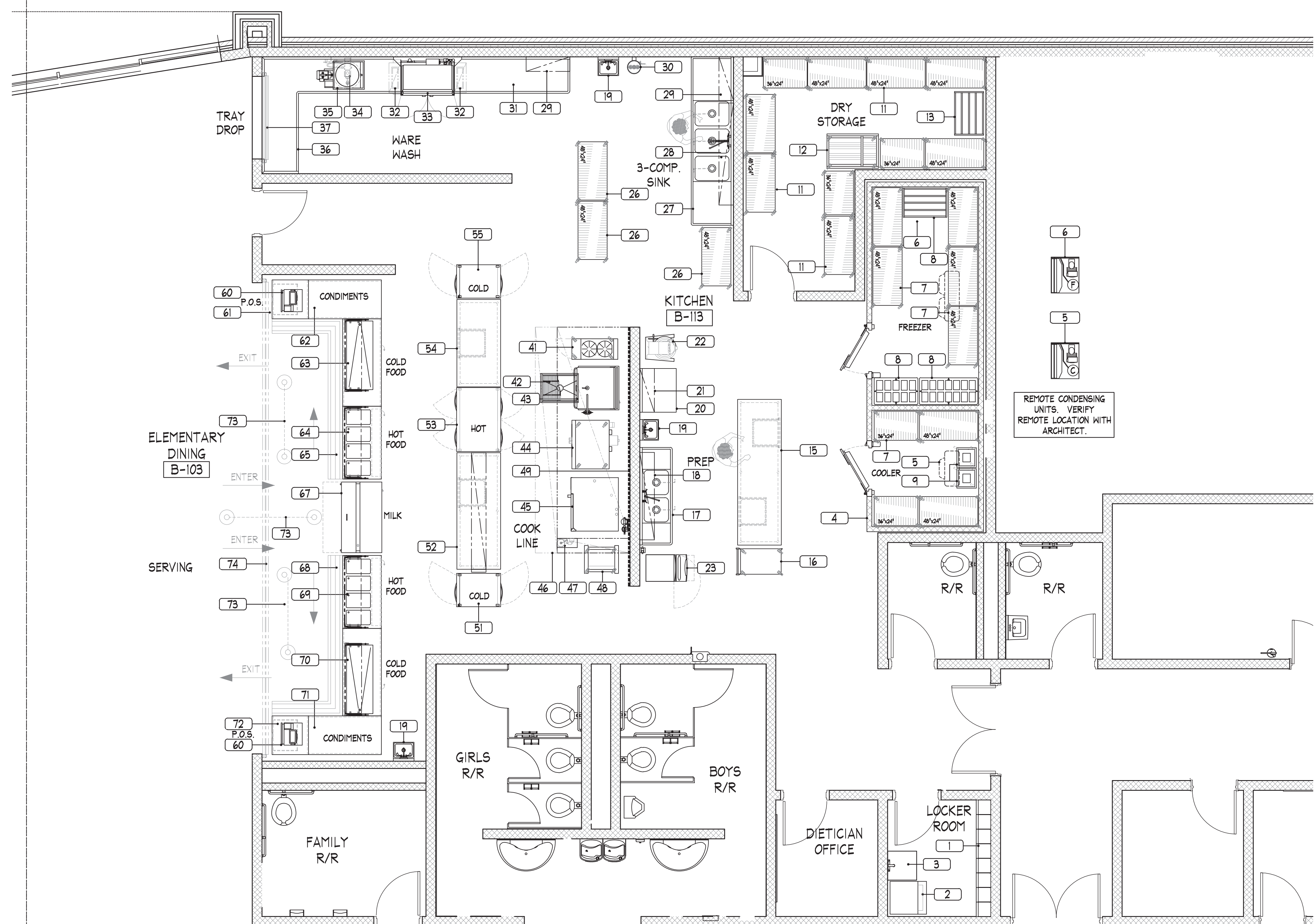
FOODSERVICE EQUIPMENT LAYOUT
