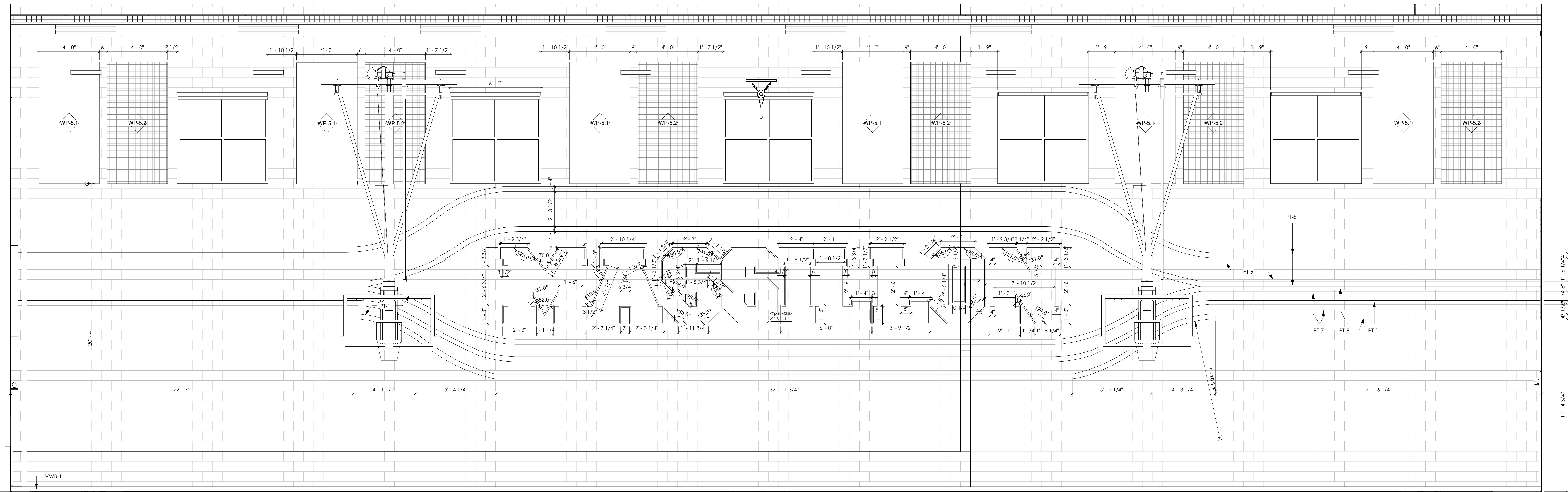
2 GYMNASIUM B-114 - WEST ELEVATION 3/8" = 1'-0"
