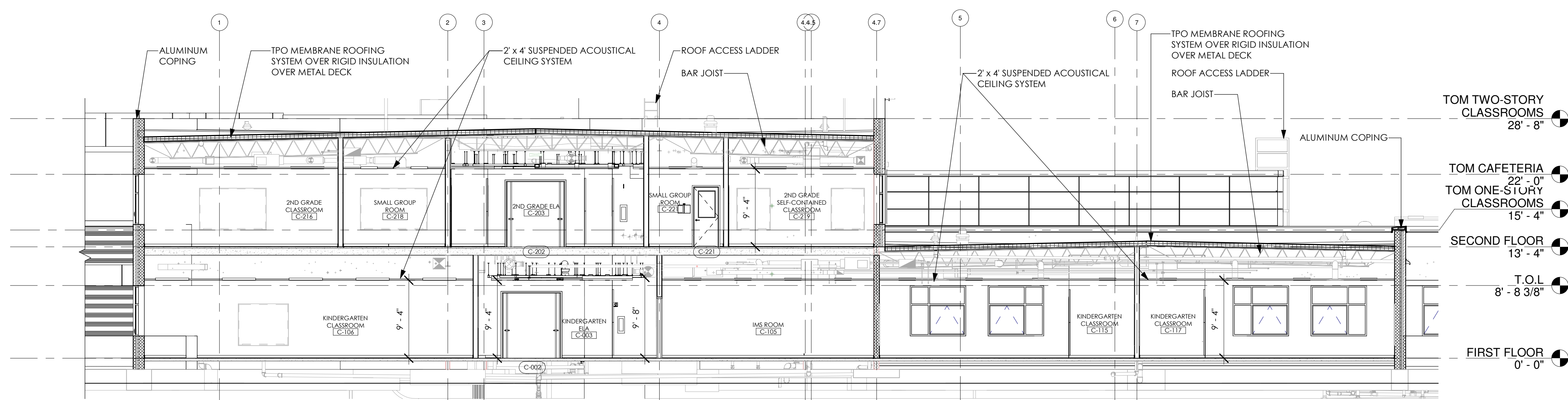
3 BUILDING SECTION 03 1/8" = 1'-0"
