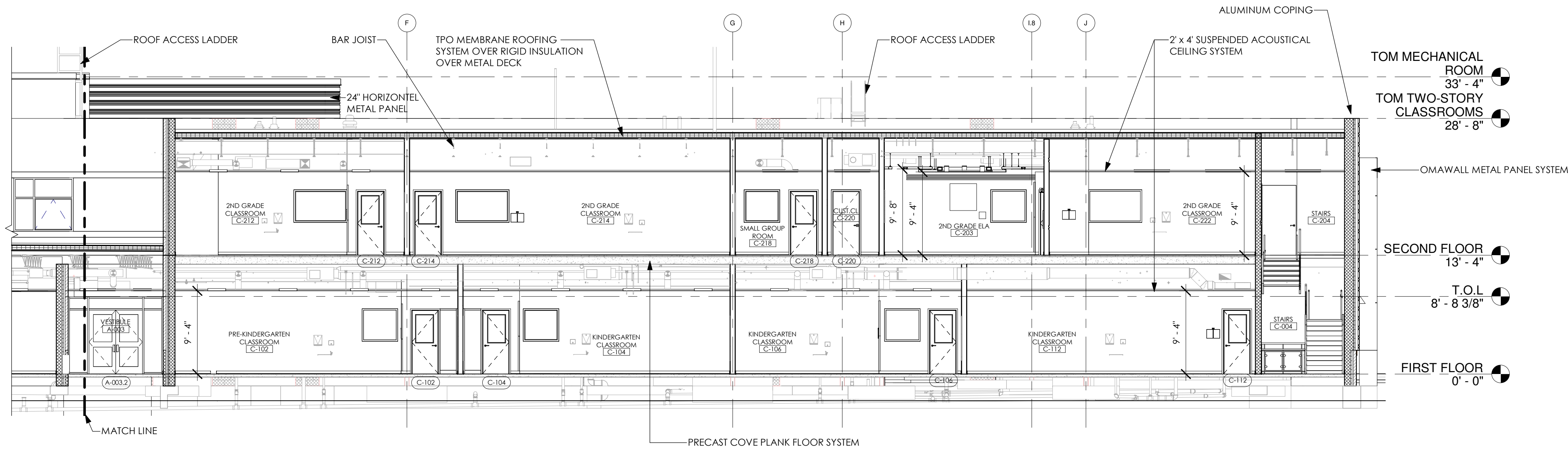
(2.1) BUILDING SECTION 02 CONT. 1/8" = 1'-0"
