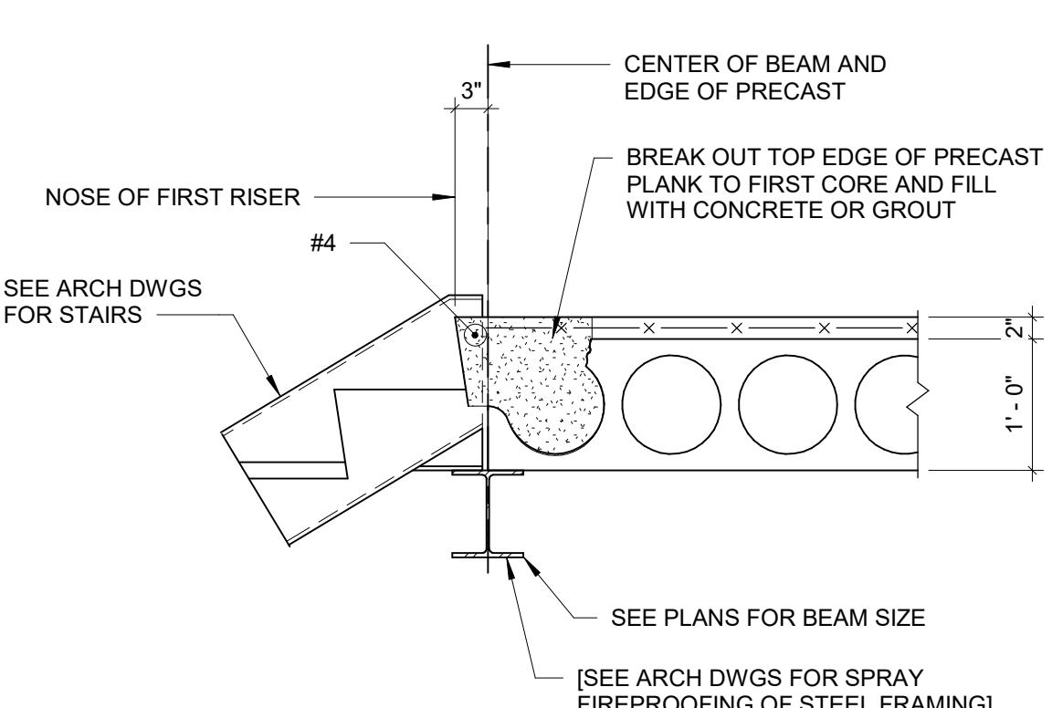
23 PRECAST PLANK AT STAIRS DETAIL SCALE: 3/4" = 1'-0"
