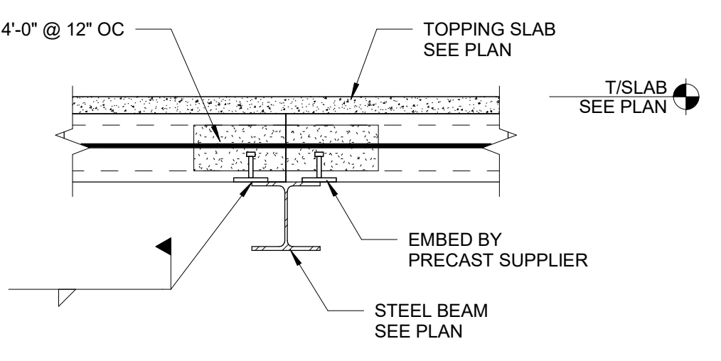
18 PLANK BEARING ON STEEL BEAM SCALE: NONE
