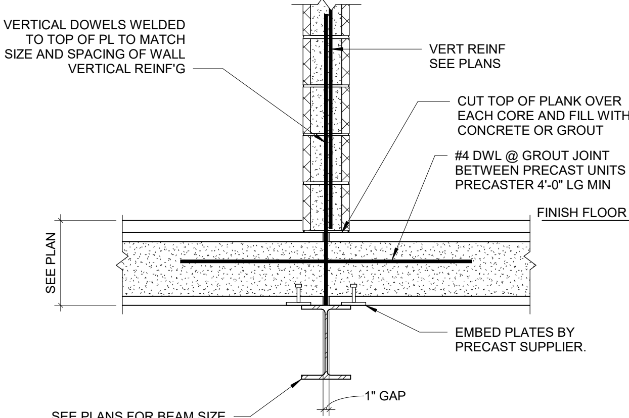
13 PRECAST PLANK STEEL CONT END BEARING W/WALL DETAIL SCALE: NONE
