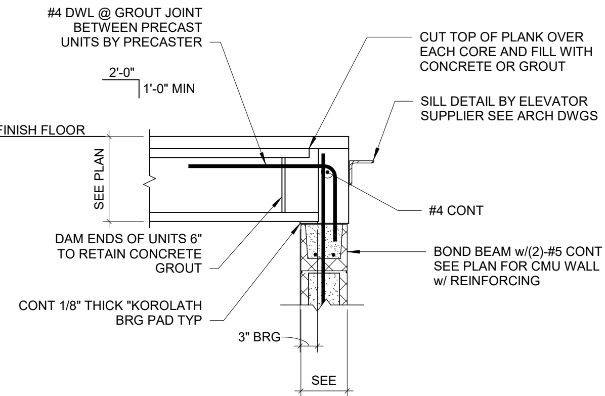
12 PRECAST PLANK/ELEVATOR SILL DETAIL SCALE: 3/4" = 1'-0"
