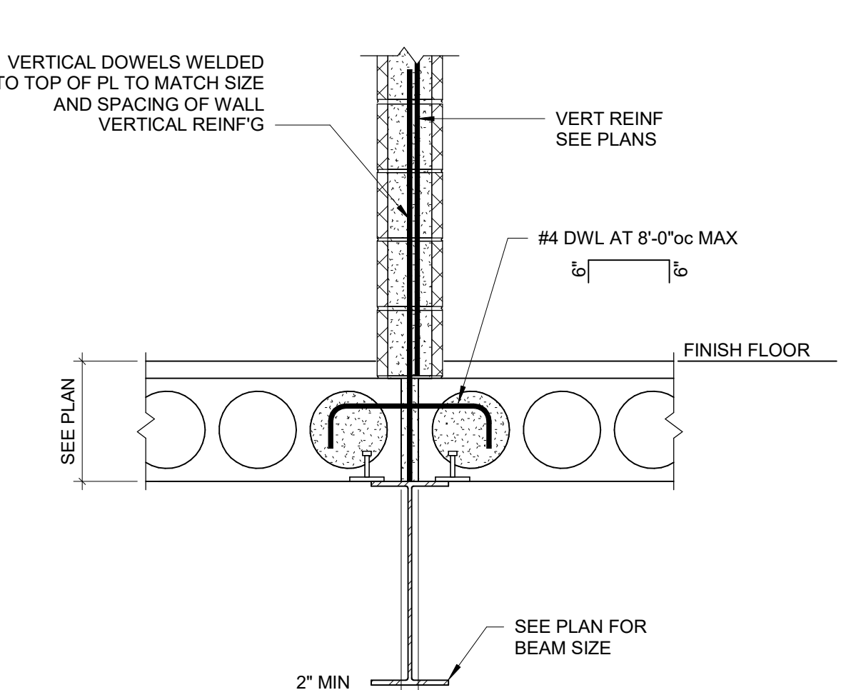
14 PRECAST PLANK STEEL CONT SIDE BEARING DETAIL SCALE: 3/4" = 1'-0"
