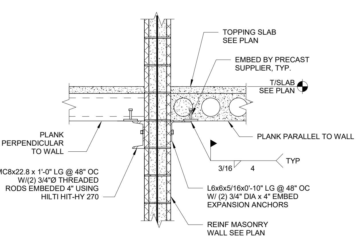
8 PLANK AT INTERIOR CMU WALL SCALE: NONE
