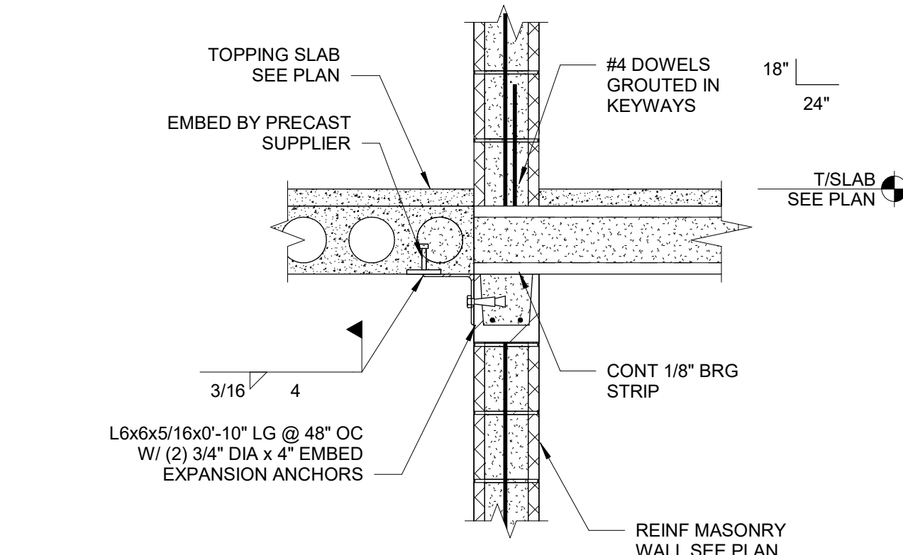
11 PLANK AT INTERIOR CMU WALL SCALE: 3/4" = 1'-0"
