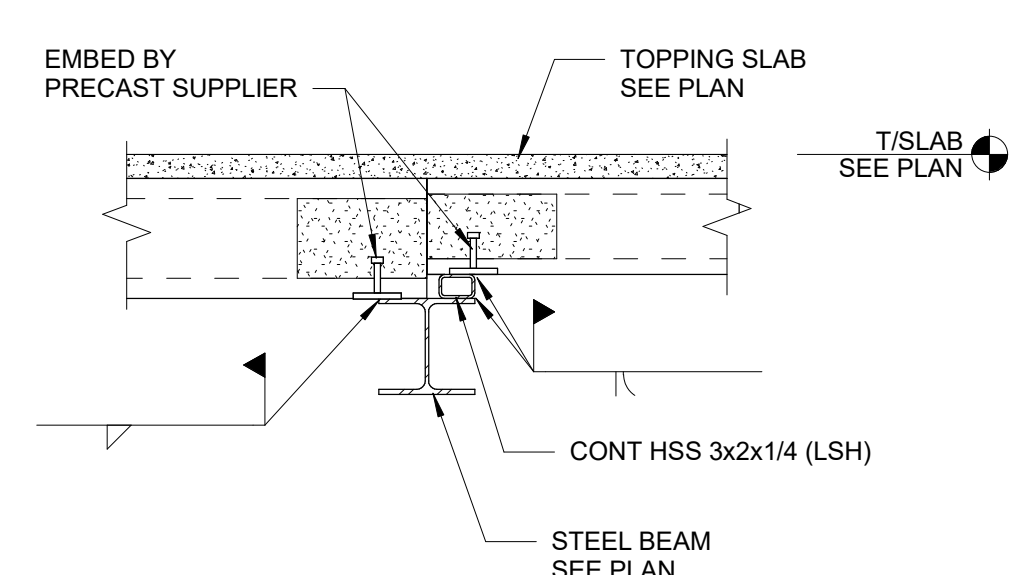
19 PLANK OF DIFFERENT THICKNESS BEARING ON STEEL BEAM SCALE: NONE
