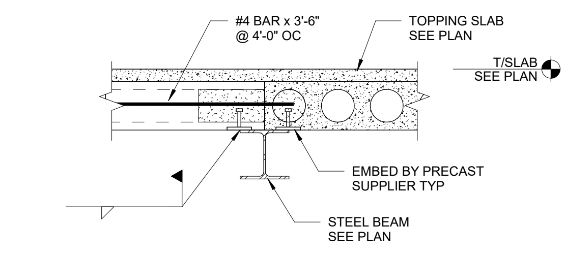
15 PLANK BEARING ON STEEL BEAM SCALE: NONE
