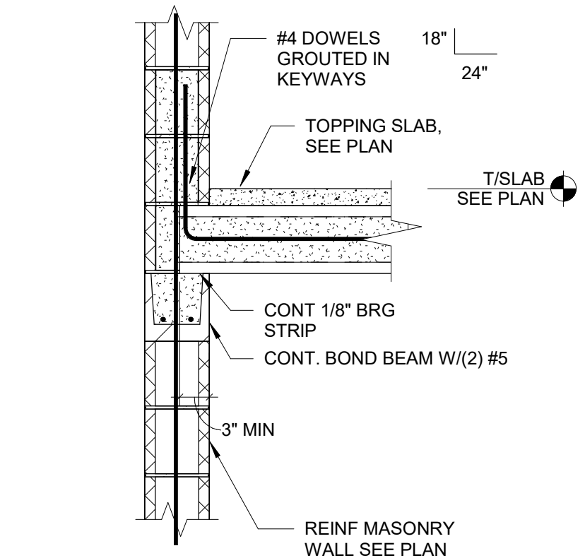
2 PLANK BEARING AT EXTERIOR CMU WALL SCALE: NONE
