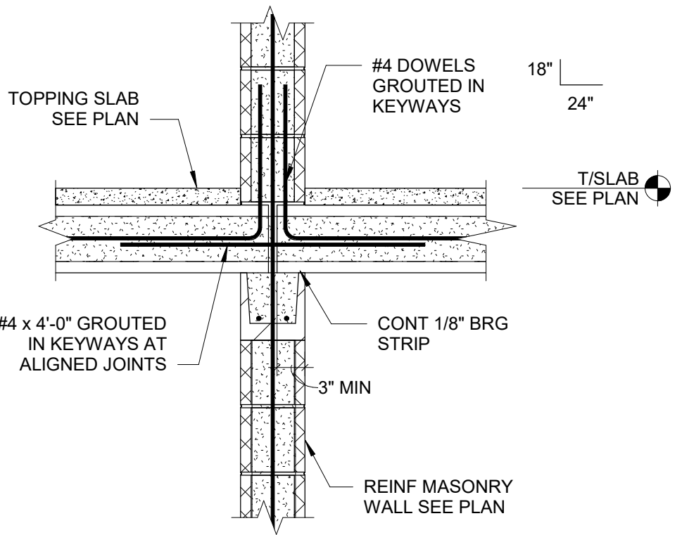
4 PLANK BEARING AT BOTH SIDES OF CMU WALL SCALE: NONE
