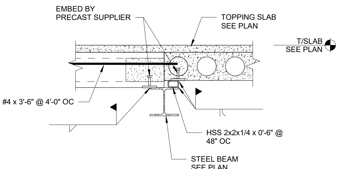
16 PLANK BEARING ON STEEL BEAM SCALE: NONE
