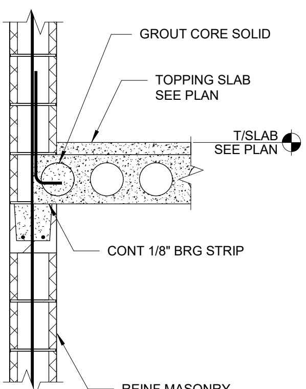
3 PLANK AT EXTERIOR CMU WALL SCALE: NONE
