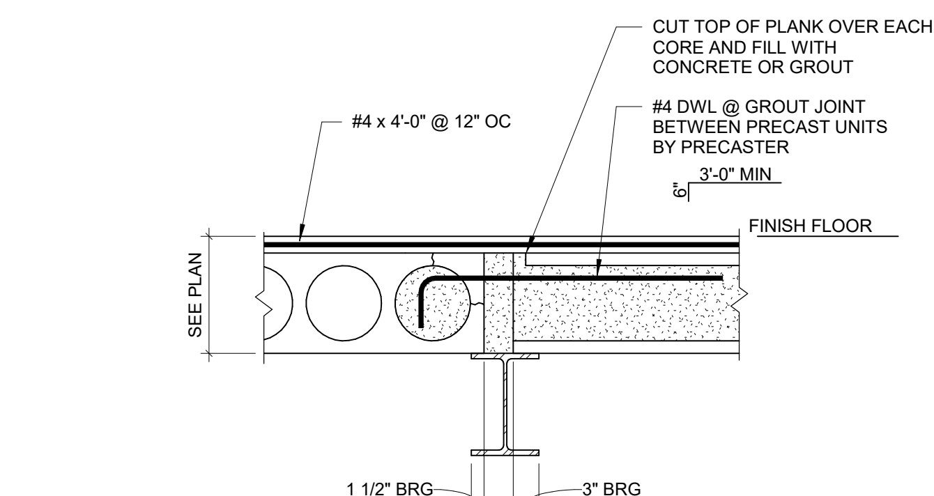
20 PRECAST PLANK STEEL SIDE AND END BEARING DETAIL SCALE: NONE
