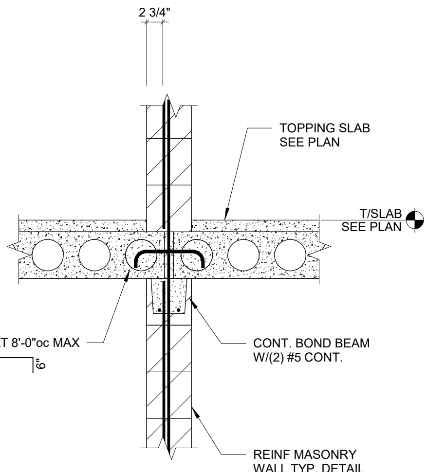
5 PLANK PARALLEL TO CMU WALL SCALE: NONE
