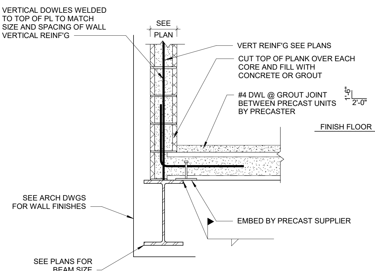
21 PRECAST PLANK STEEL END BEARING W/WALL DETAIL SCALE: NONE
