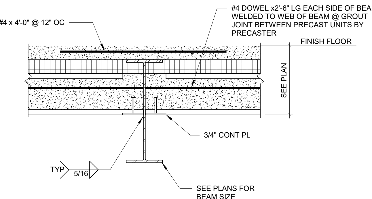
22 PRECAST PLANK FLUSH STEEL CONT END BEARING DETAIL SCALE: 3/4" = 1'-0"
