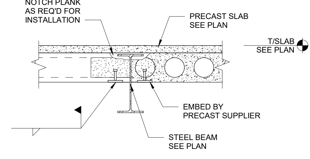
24 PLANK BEARING ON STEEL BEAM SCALE: 3/4" = 1'-0"
