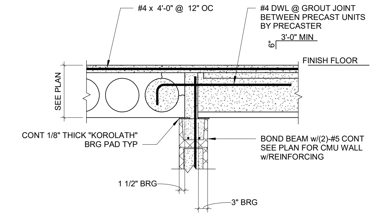
9 PRECAST PLANK CMU SIDE AND END BEARING DETAIL SCALE: NONE
