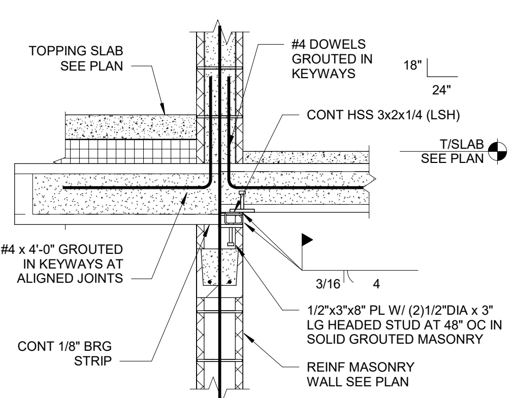
10 PLANK OF DIFFERENT THICKNESS AT INTERIOR CMU WALL SCALE: NONE
