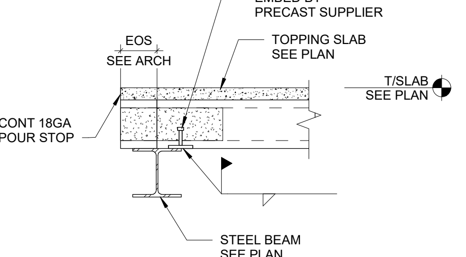
17 PLANK BEARING ON STEEL BEAM SCALE: NONE
