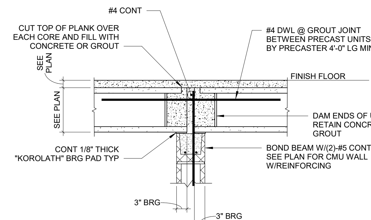
6 PRECAST PLANK CONTINUOUS CMU END BEARING DETAIL SCALE: 3/4" = 1'-0"
