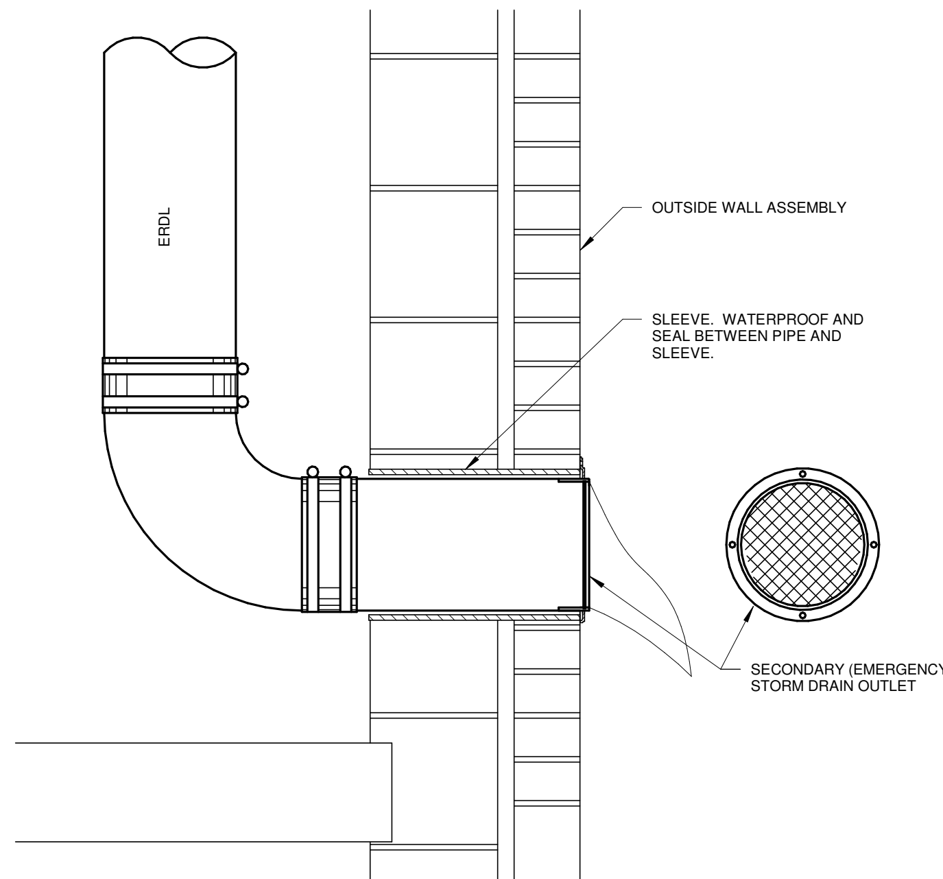
EMERGENCY STORM DRAIN OUTLET DETAIL N.T.S.
