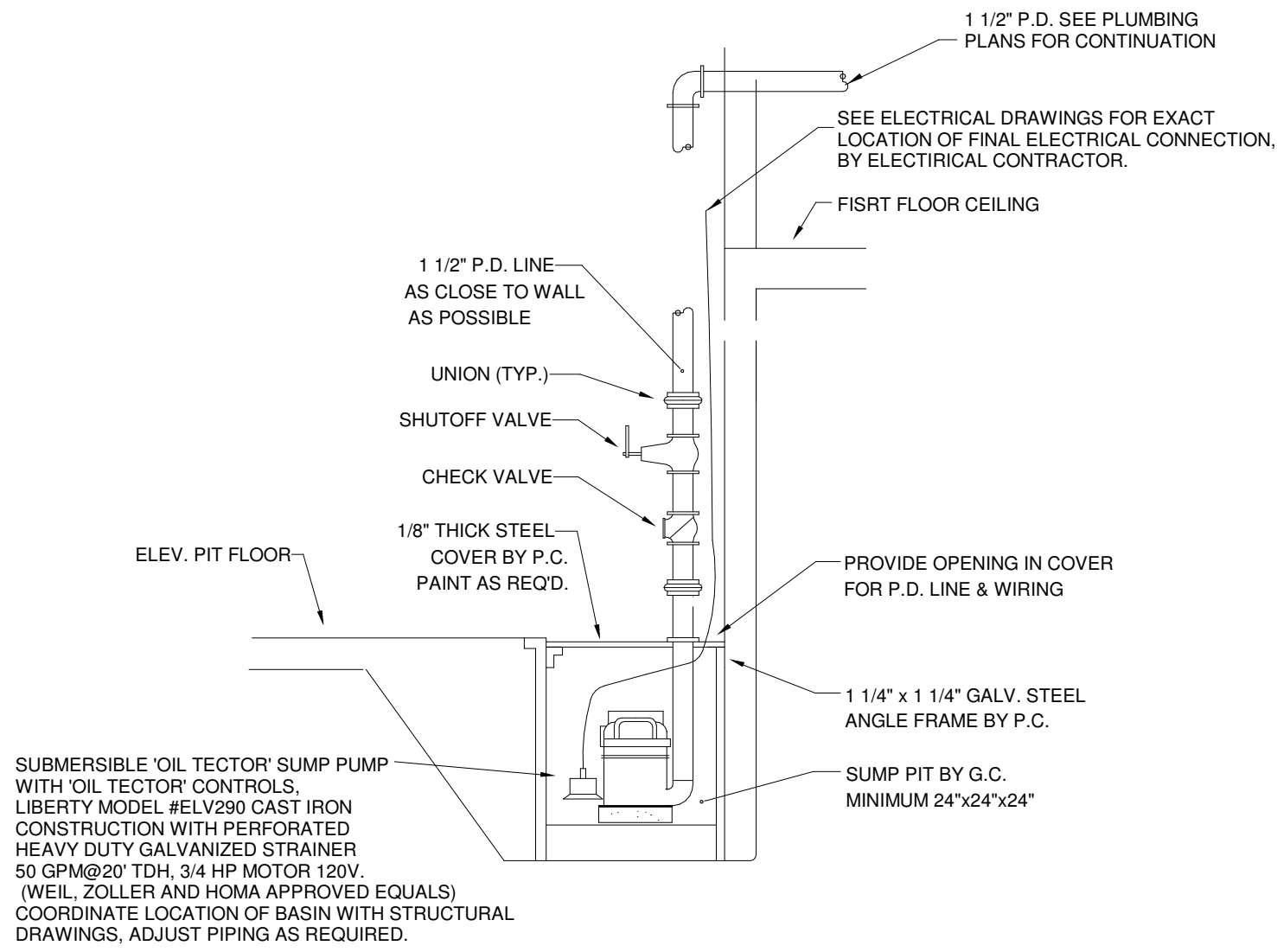
ELEVATOR PIT SUMP PUMP DETAIL N.T.S.
