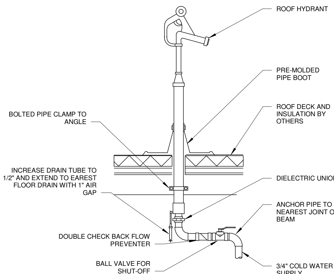
ROOF HYDRANT DETAIL N.T.S.
