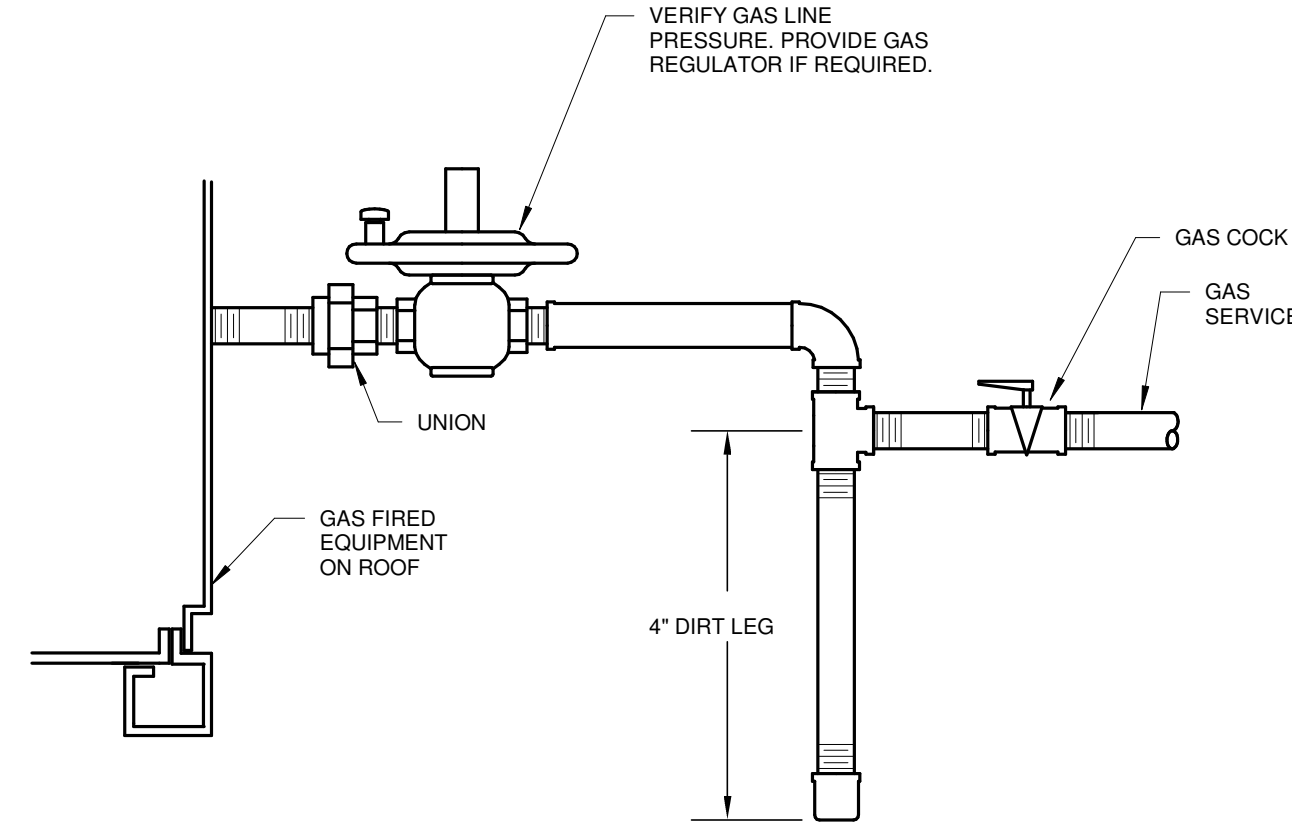
GAS CONNECTION TO EQUIPMENT ON ROOF DETAIL N.T.S.
