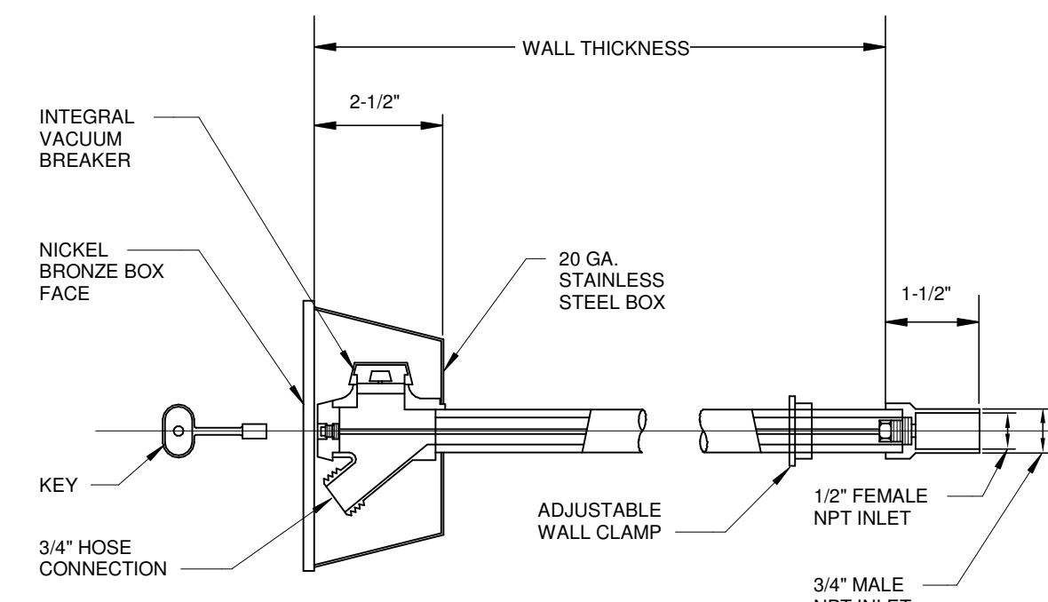
NON-FREEZE WALL HYDRANT DETAIL N.T.S.
