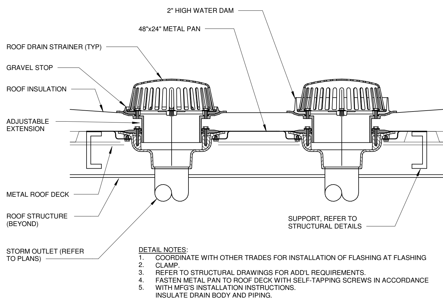
STORM AND OVERFLOW ROOF DRAIN DETAIL N.T.S.
