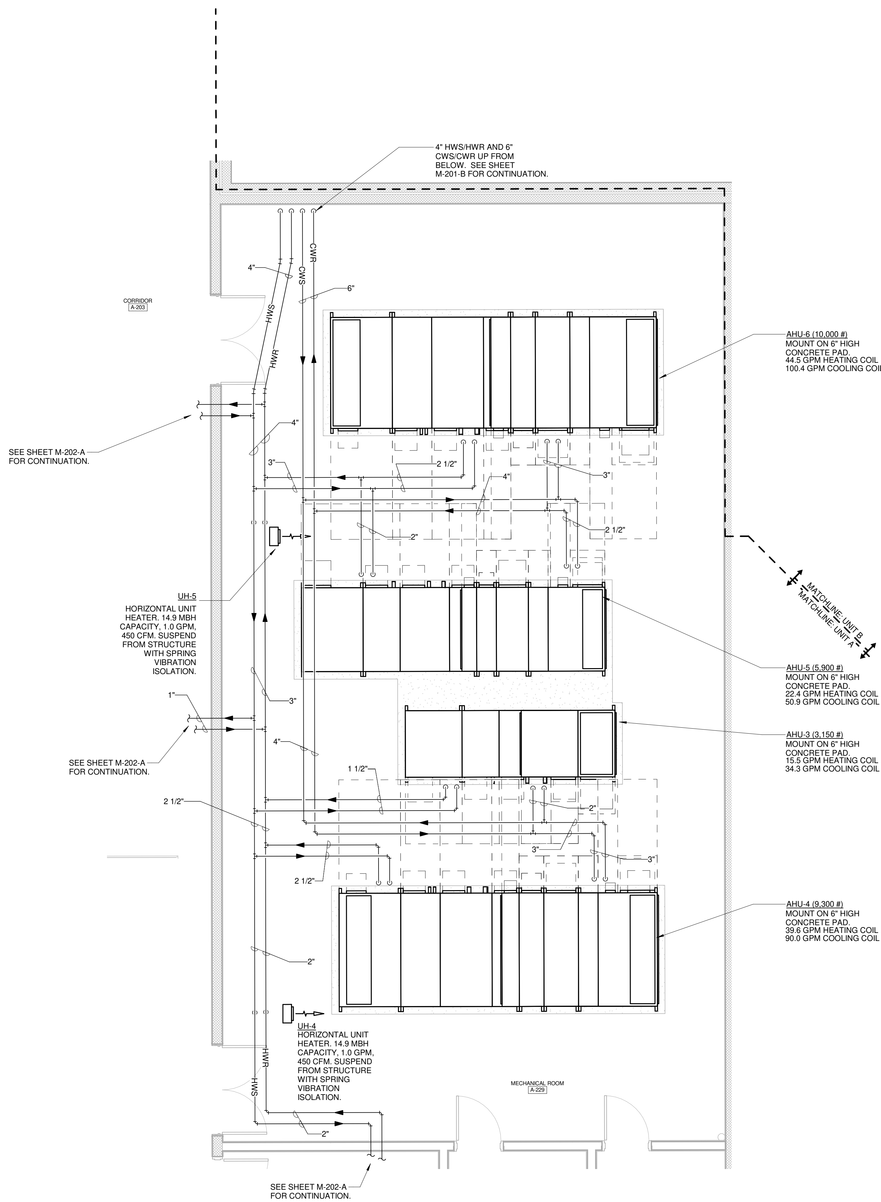
PARTIAL SECOND FLOOR PLAN - ENLARGED MECH ROOM A-229 - HVAC PIPING SCALE: 1/4" = 1'-0"
