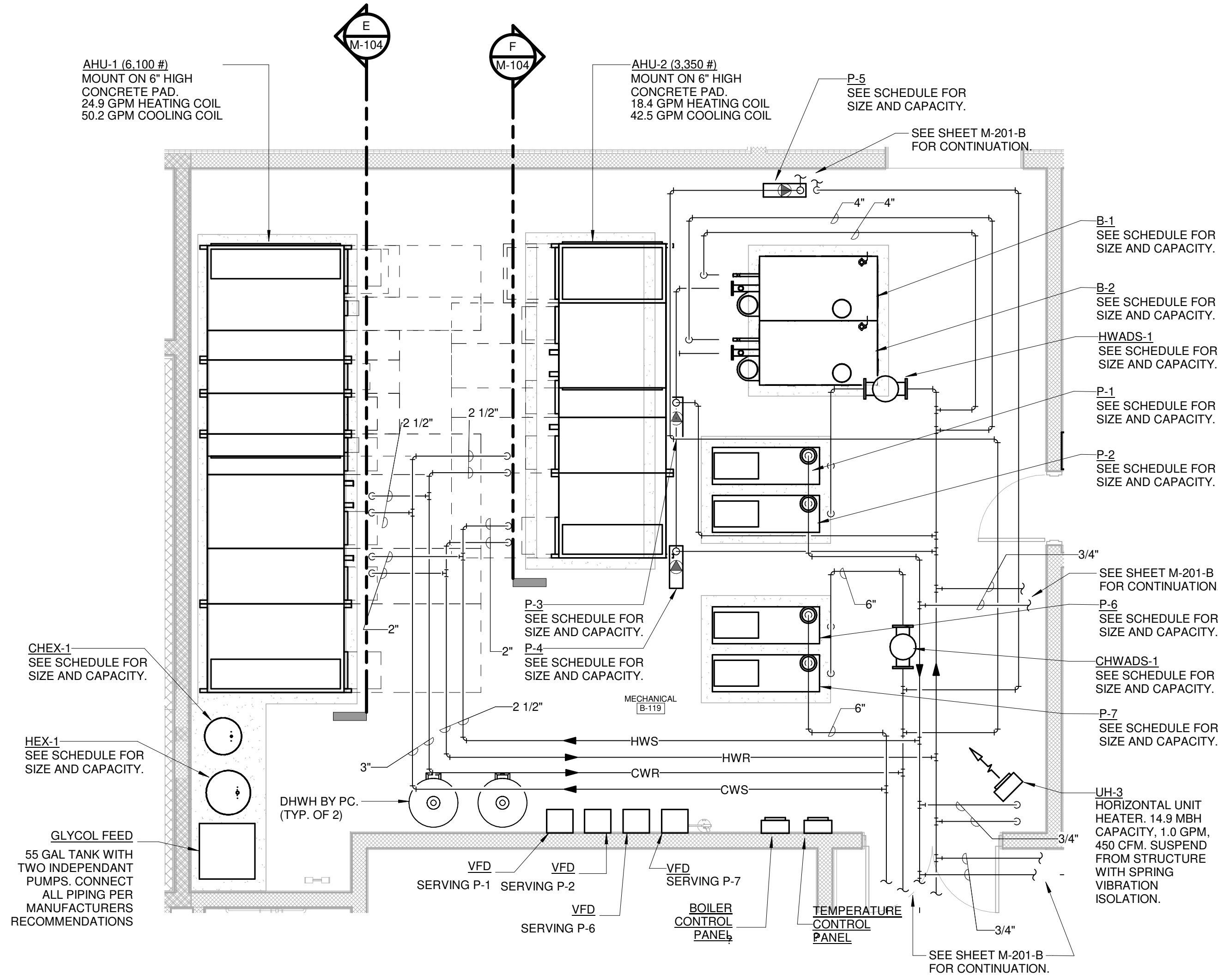
PARTIAL FIRST FLOOR PLAN - ENLARGED MECH ROOM B-119 - HVAC PIPING SCALE: 1/4" = 1'-0"
