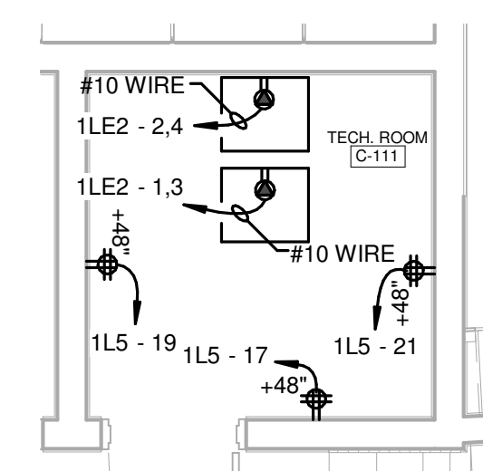
ENLARGED TECH ROOM C-111 - POWER SCALE: 1/4" = 1'-0"
