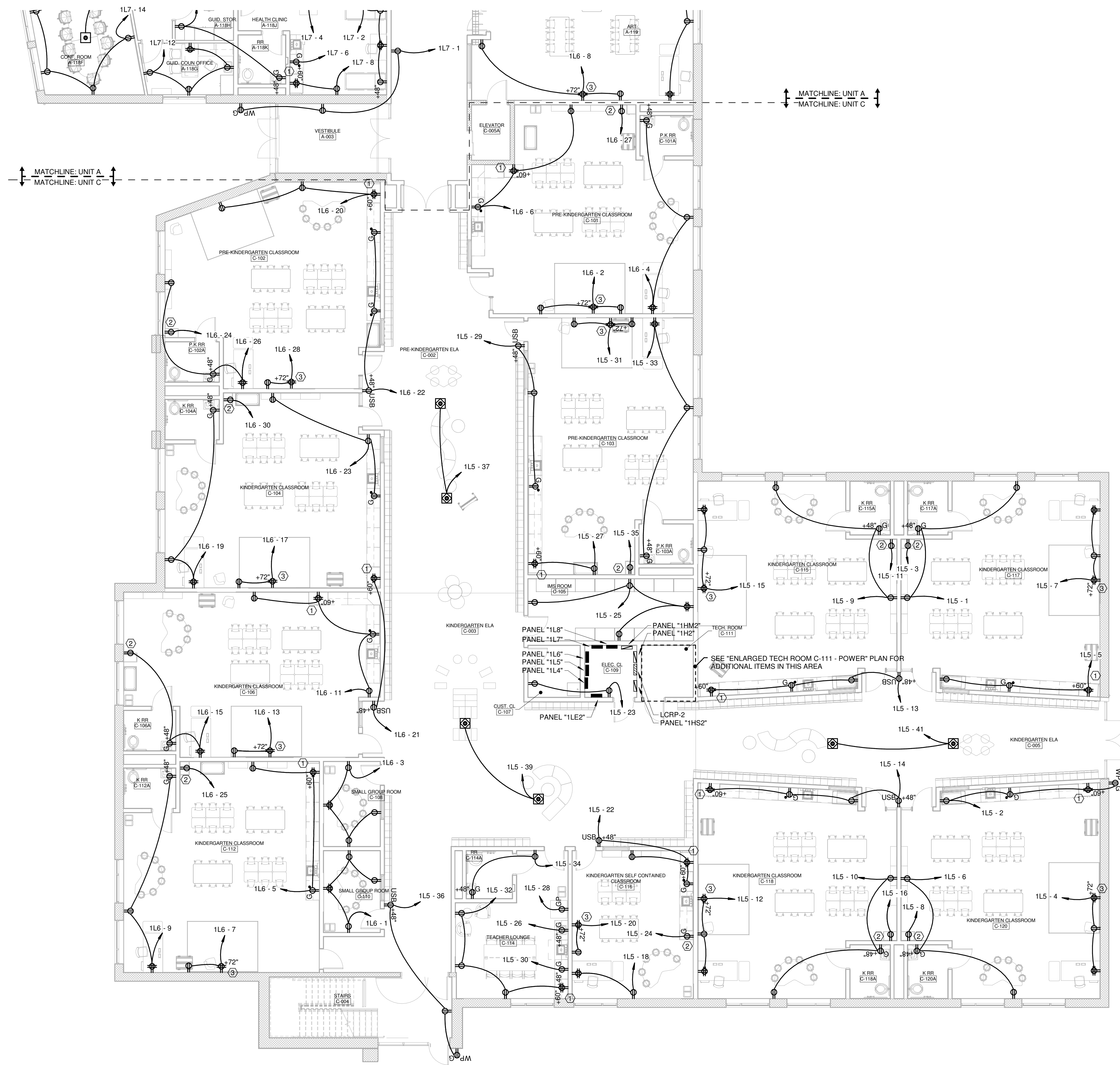
FIRST FLOOR PLAN - POWER - UNIT C SCALE: 1/8" = 1'-0"
