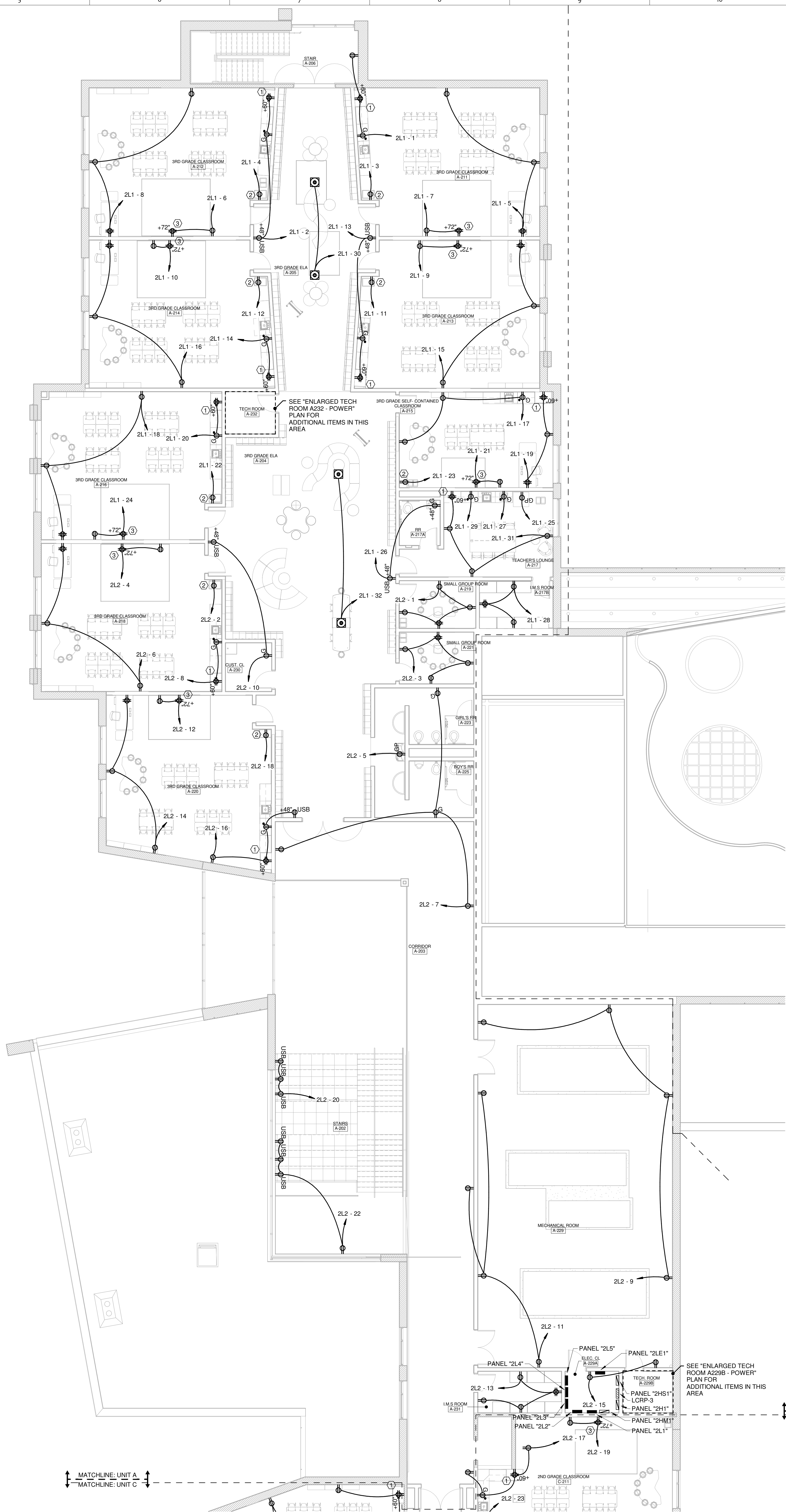
SECOND FLOOR PLAN - POWER - UNIT A SCALE: 1/8" = 1'-0"
