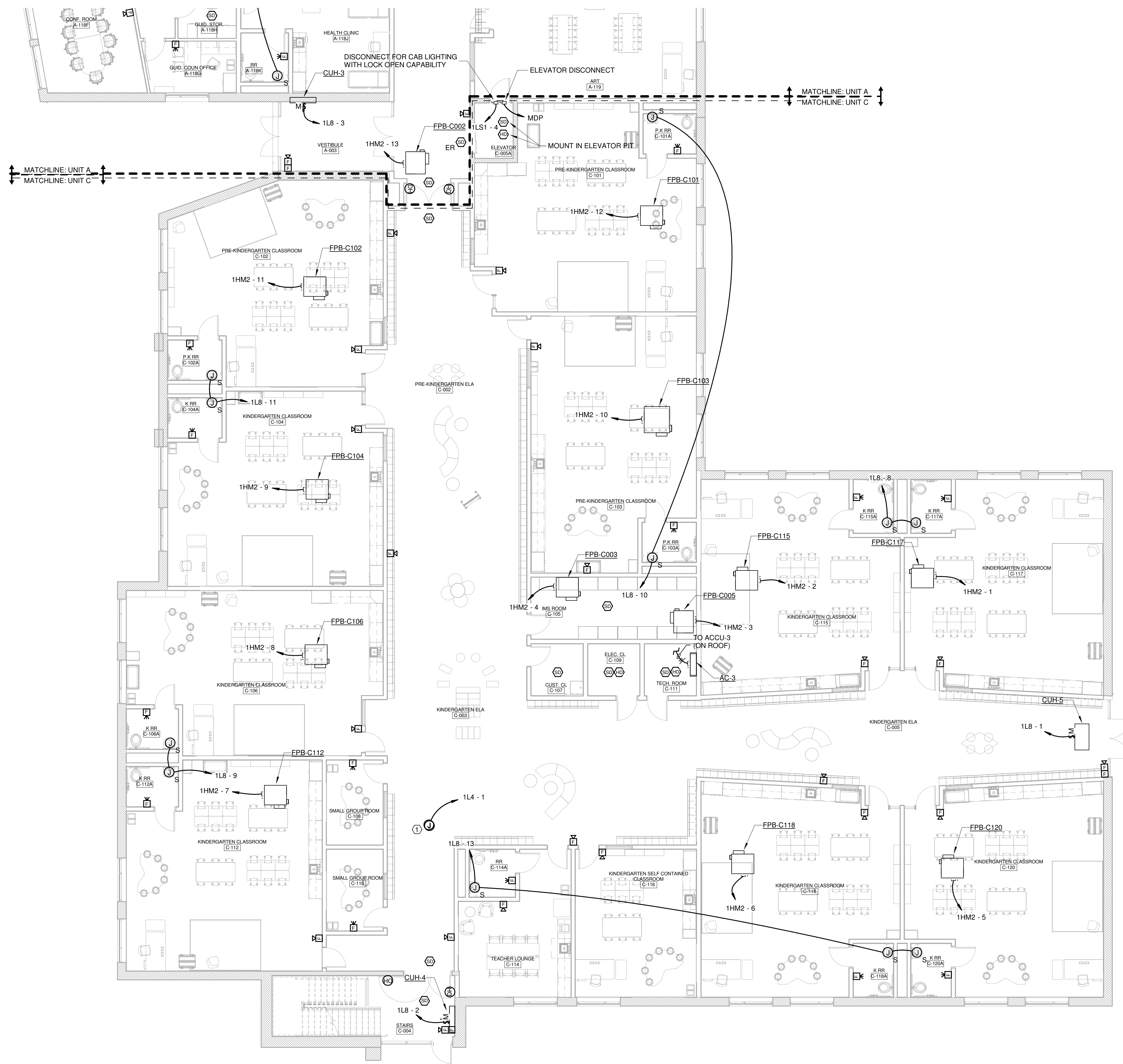
FIRST FLOOR PLAN - SYSTEMS - UNIT C SCALE: 1/8" = 1'-0"
