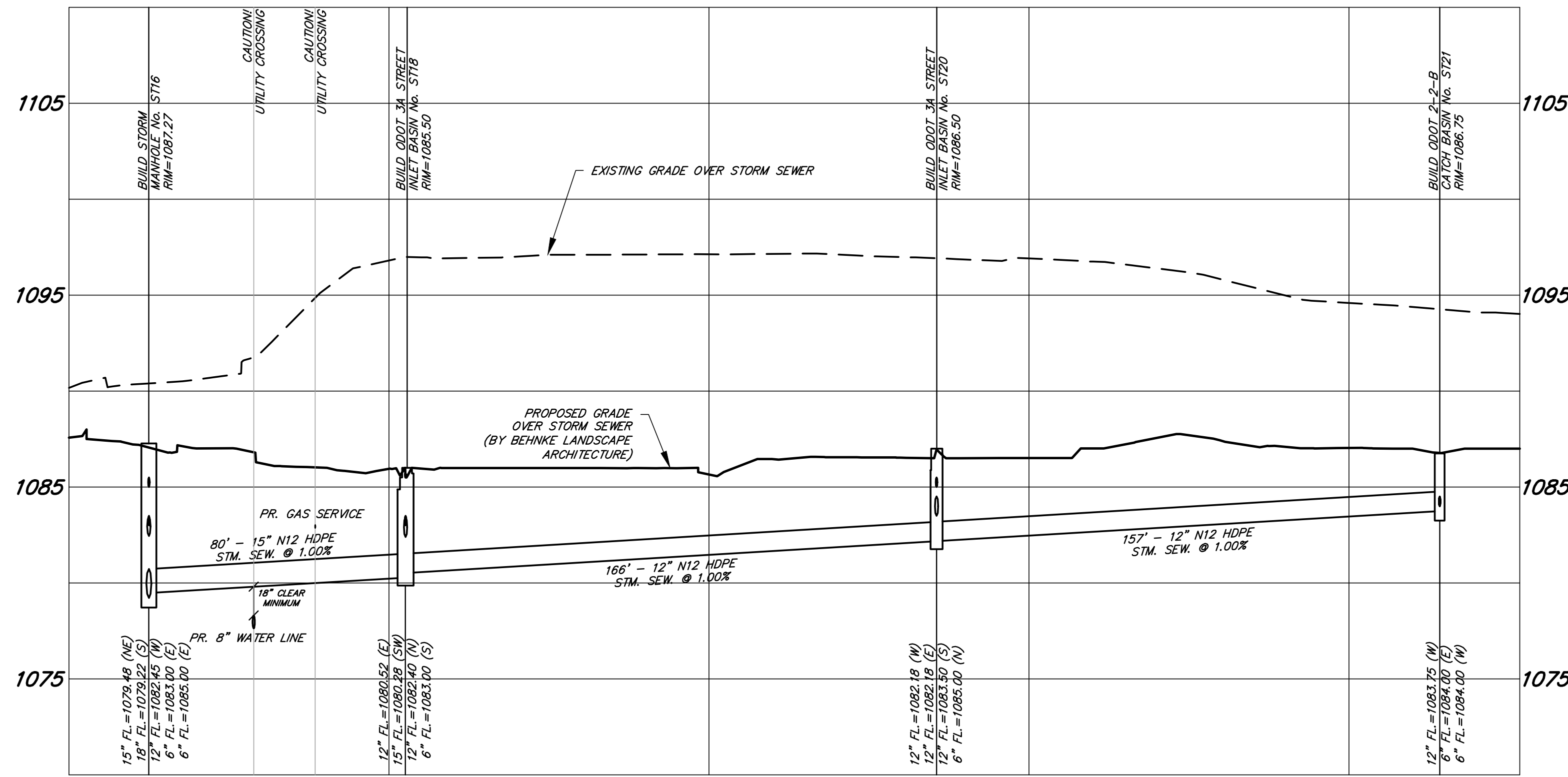
STORM SEWER PROFILE ST21 TO ST26 SCALE: HORIZ. 1"=30', VERT. 1"=5'
