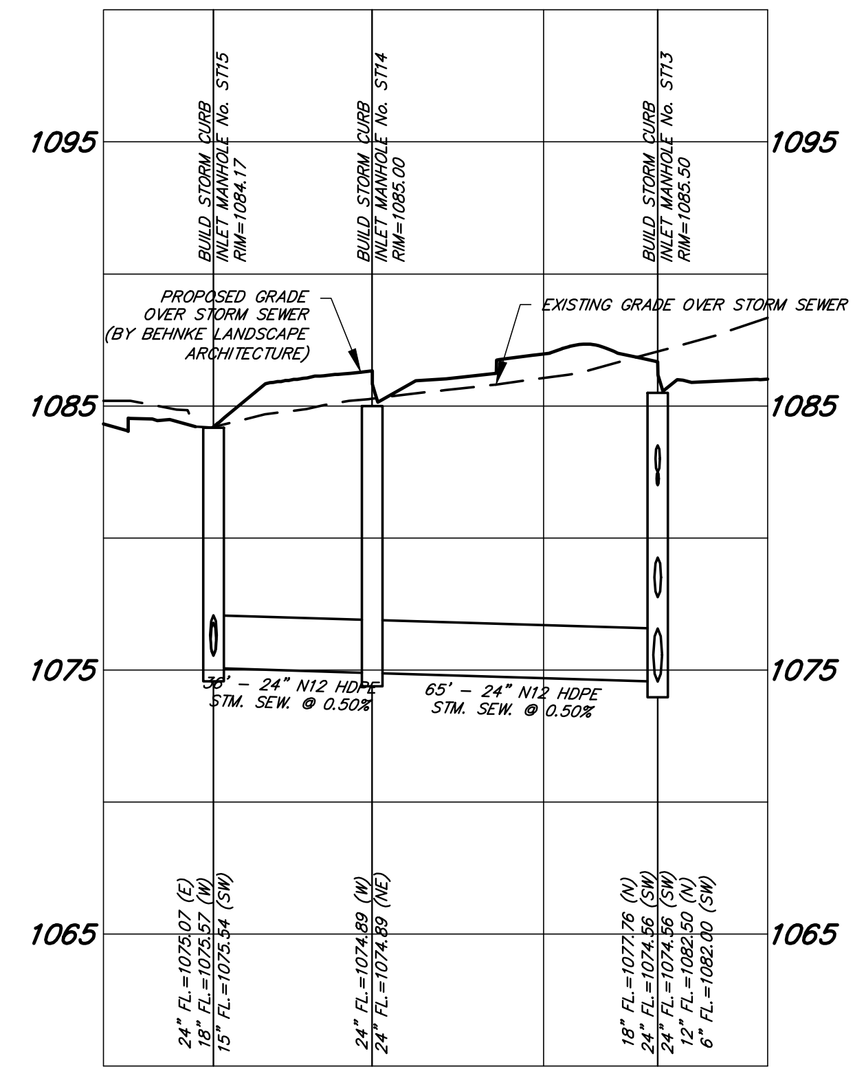
STORM SEWER PROFILE ST13 TO ST15 SCALE: HORIZ. 1"=30', VERT. 1"=5'
