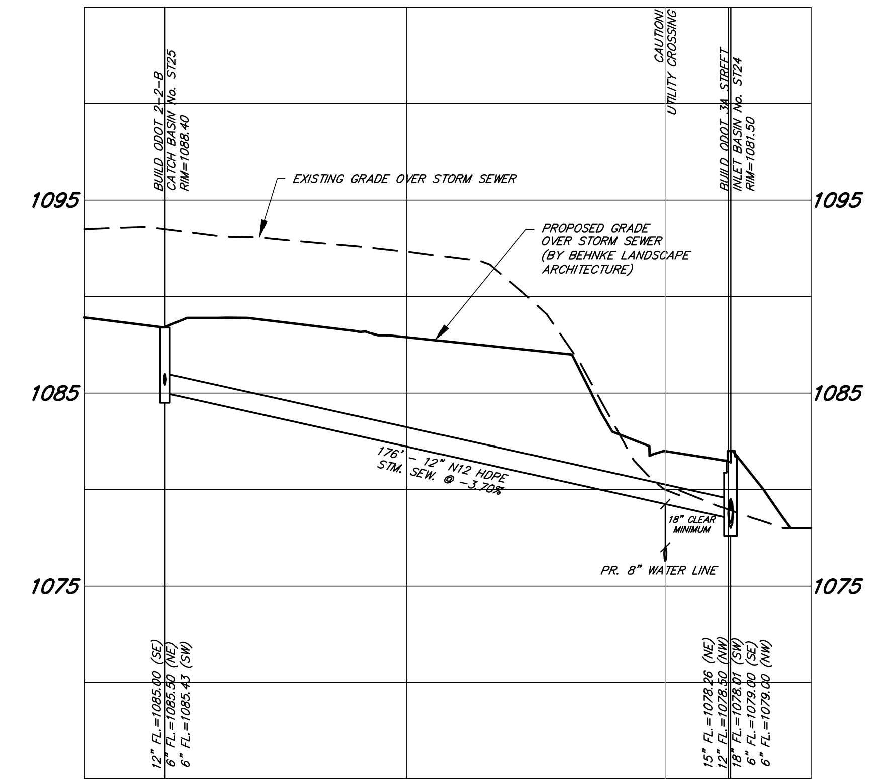
STORM SEWER PROFILE ST25 TO ST24 SCALE: HORIZ. 1"=30', VERT. 1"=5'
