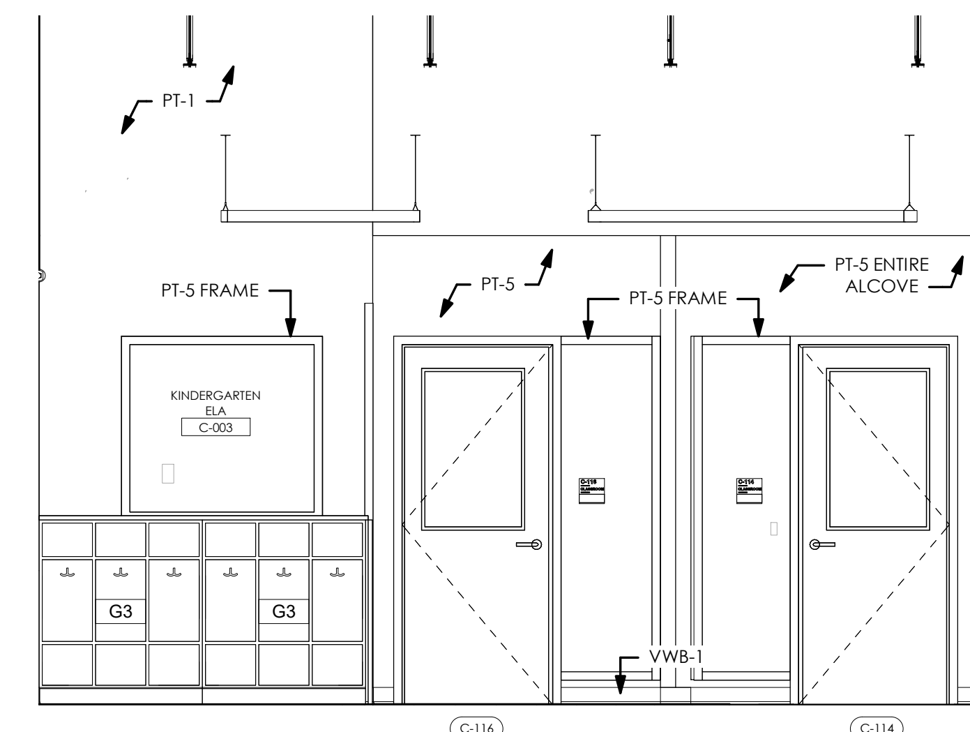
9 KINDERGARTEN ELA C-003 - WEST ELEVATION 2 3/8" = 1'-0"
