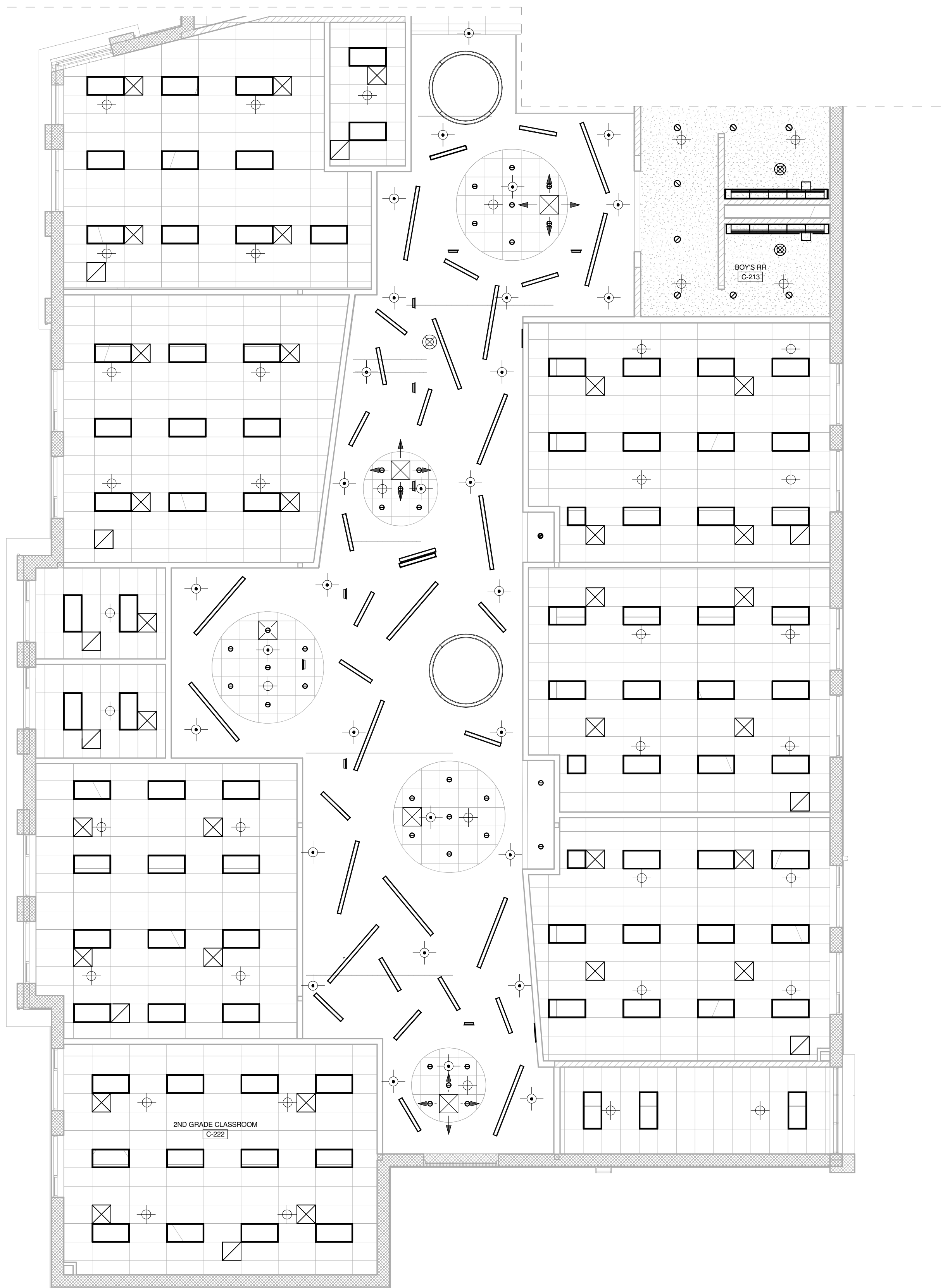
SECOND FLOOR PLAN - FIRE PROTECTION - UNIT C SCALE: 1/8" = 1'-0"
