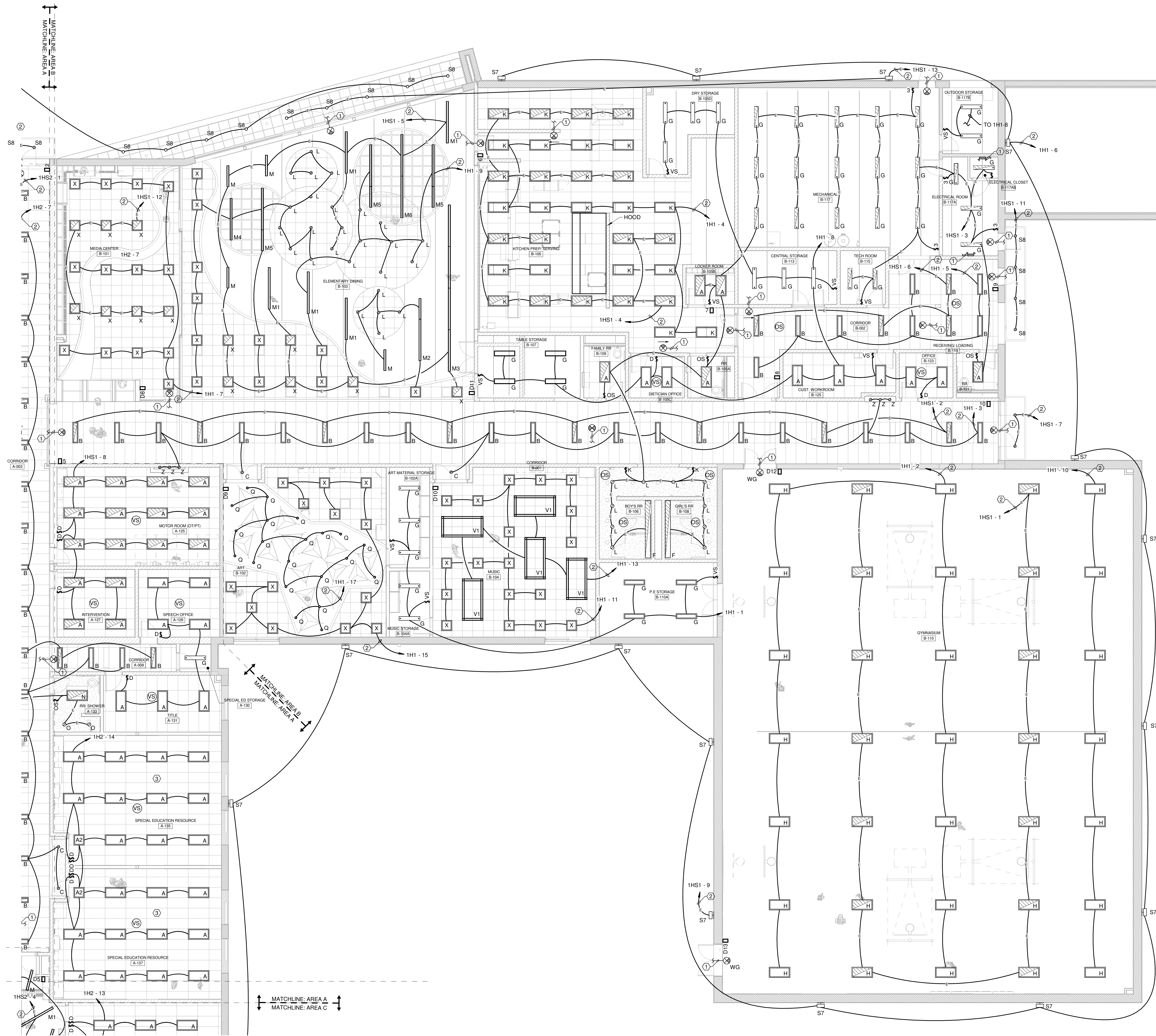
FIRST FLOOR PLAN - LIGHTING - UNIT B SCALE: 1/8" = 1'-0"
