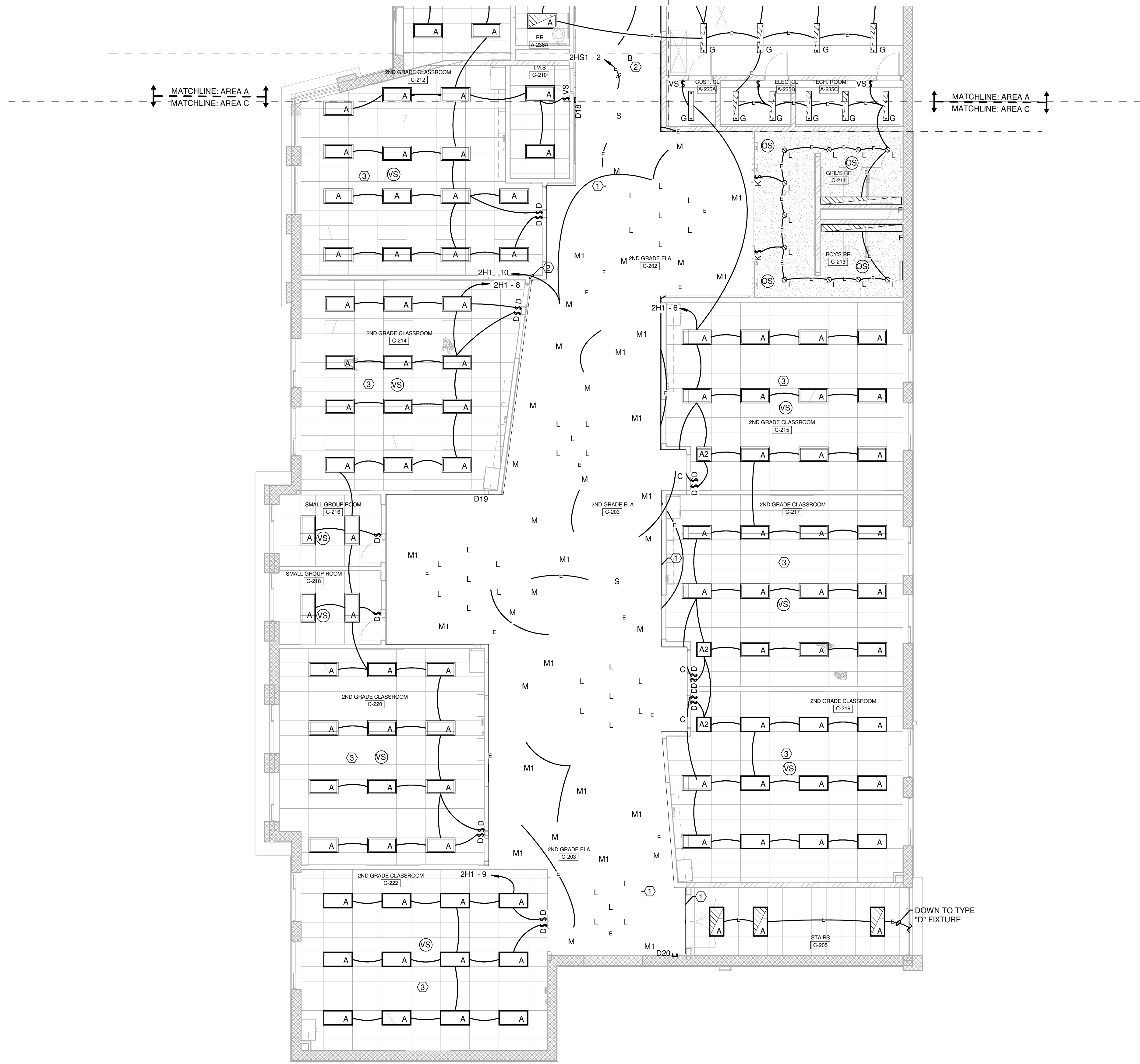
SECOND FLOOR PLAN - LIGHTING - UNIT C SCALE: 1/8" = 1'-0"
