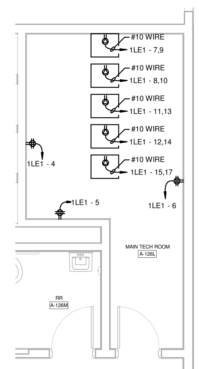
ENLARGED MAIN TECH ROOM A-126L SCALE: 1/4" = 1'-0"
