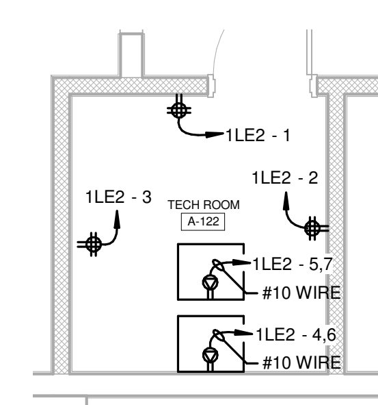
ENLARGED TECH ROOM A-122 - POWER SCALE: 1/4" = 1'-0"
