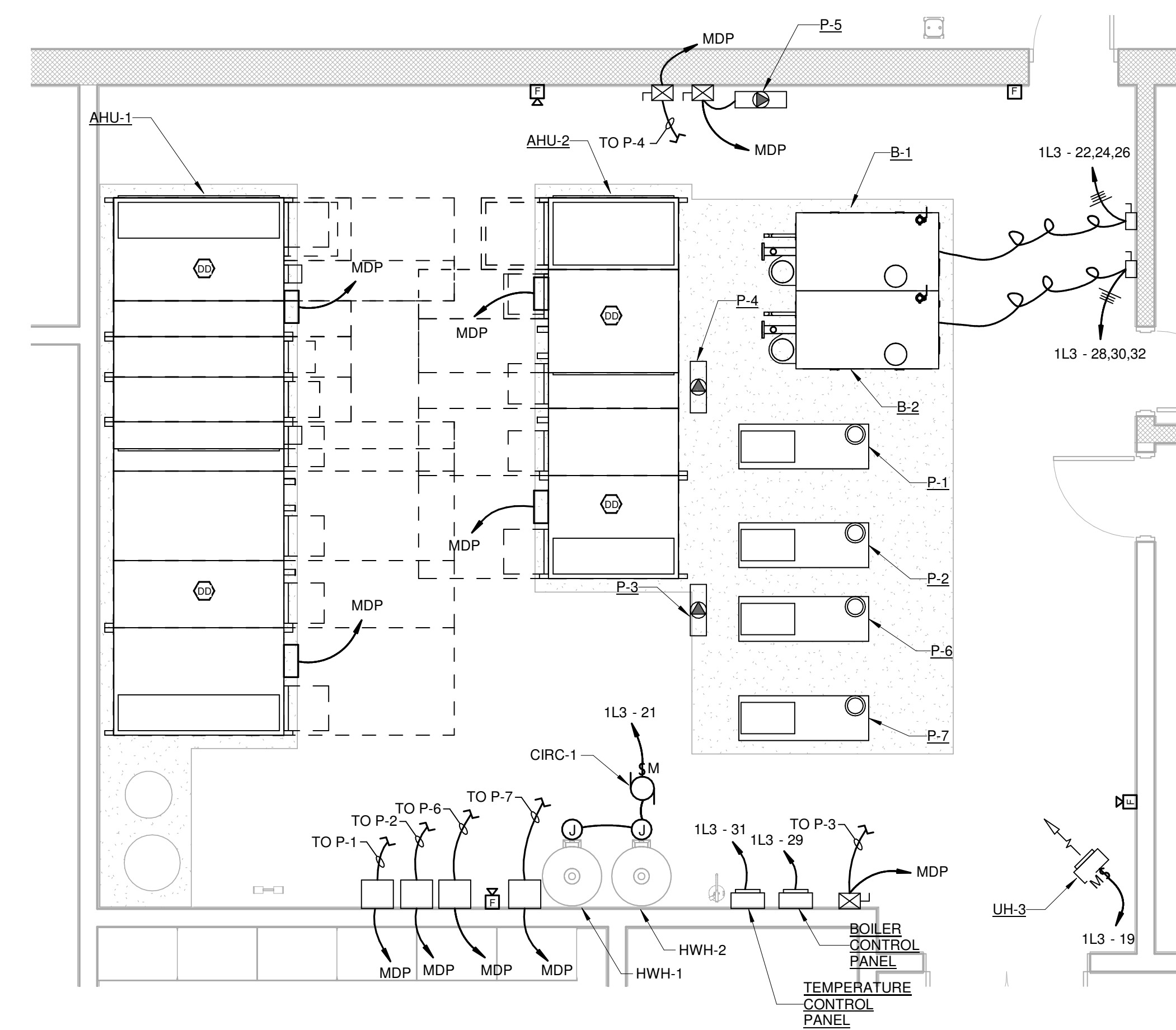
ENLARGED MECHANICAL ROOM B-117 SCALE: 1/4" = 1'-0"
