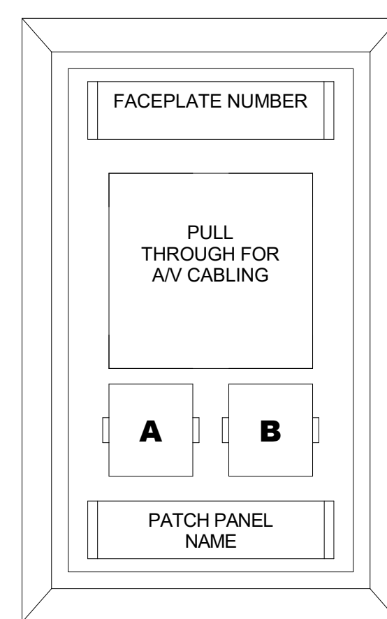
TYPE "V" AVC FACEPLATE DETAIL SCALE: NONE
