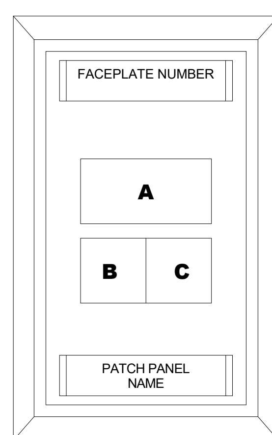
TYPE "T" "T" FACEPLATE DETAIL SCALE: NONE
