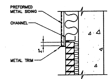
METAL SIDING OVERHANG DETAIL SCALE: 1"=1'-0"
