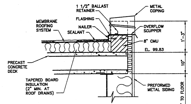
OVERFLOW SCUPPER DETAIL SCALE: 1"=1'-0"
