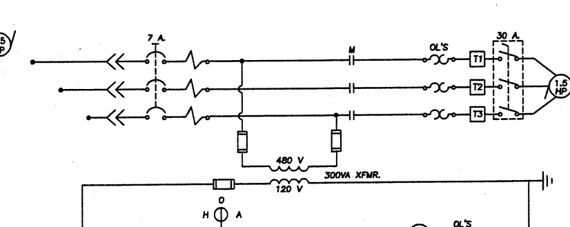
EXHAUST FAN EF-2 (TERTIARY FILTER AND UV DISINFECTION BUILDING)
