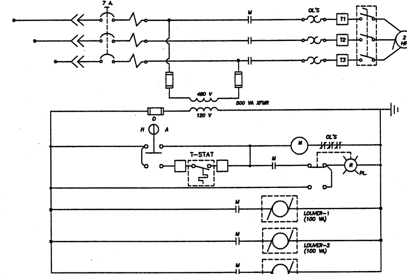
EXHAUST FAN EF-1 (TERTIARY FILTER AND UV DISINFECTION BUILDING)
