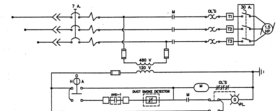
EXHAUST FAN EF-1 (SCREEN AND PUMP BUILDING)
