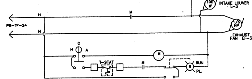
EXHAUST FAN EF-3 (TERTIARY FILTER AND UV DISINFECTION BUILDING)
