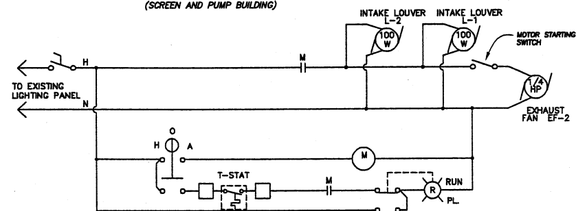
EXHAUST FAN EF-2 (SCREEN AND PUMP BUILDING)
