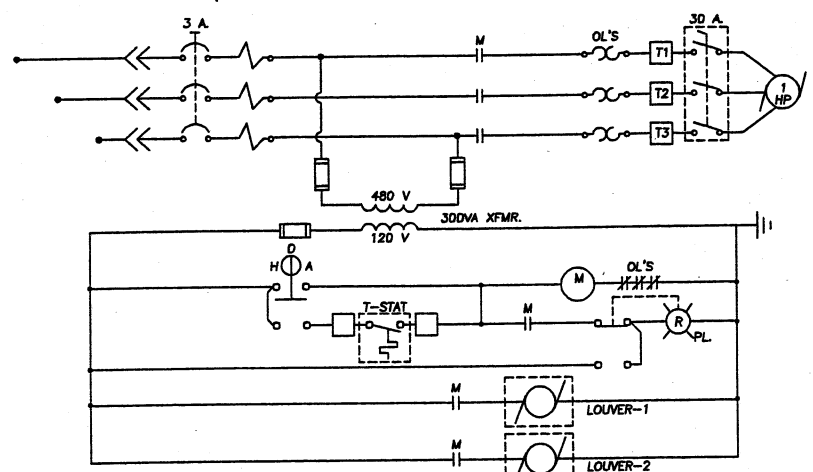
EXHAUST FAN EF-1 (SOLIDS HANDLING BUILDING ADDITION)
