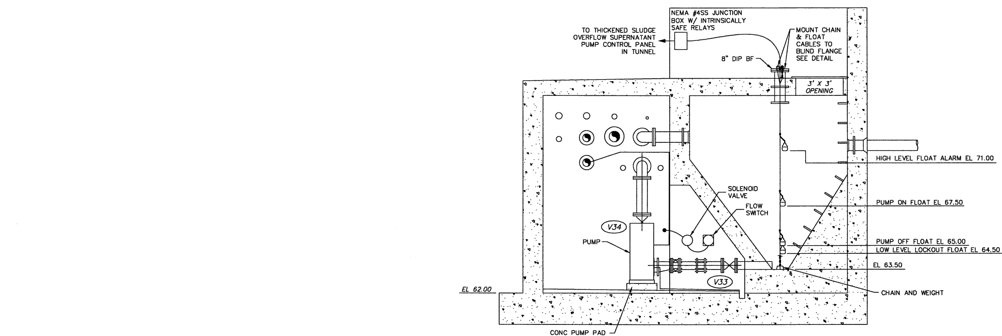
SECTION SCALE : 3/8"=1'-0" (B)
