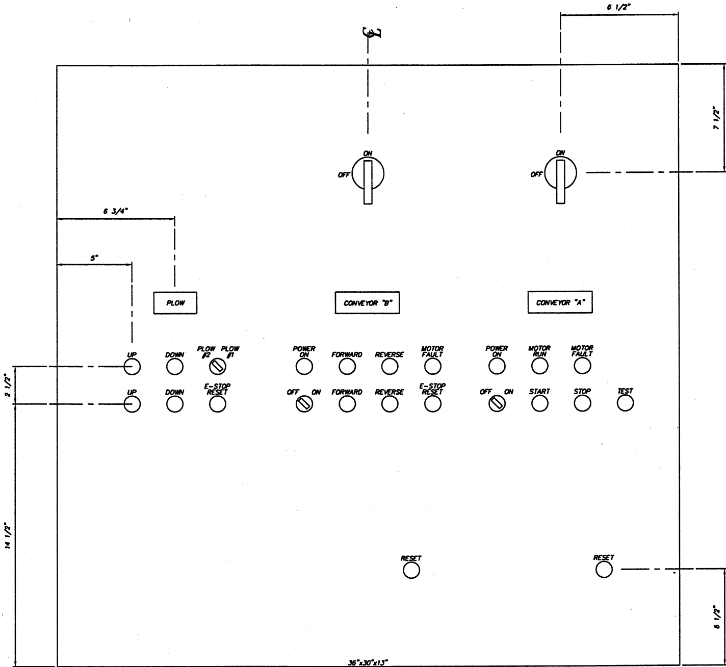
CONVEYOR BELT CONTROL CENTER LOCATED AT TOP OF STAIRS IN SOLIDS HANDLING BLDG. ADDITION (SEE DRAWING P-91)
