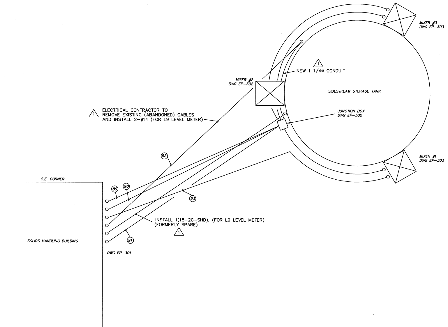
CABINET LAYOUT OF SIDESTREAM STORAGE TANK NTS
