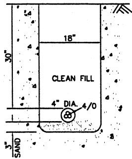
DETAIL "A" SUGGESTED UG CABLE INSTALLATION OR INSTALL AS PER N.E.C. (TYPICAL FOR UG CABLE INSTALLATIONS)
