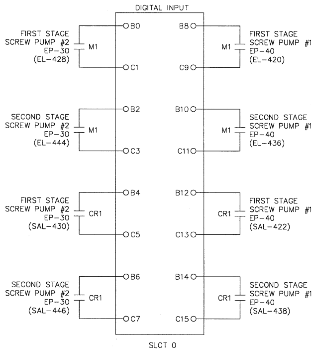
NODE 3: TRANSFORMER "B & C" - SCREW PUMPS & AERATION MIXERS
