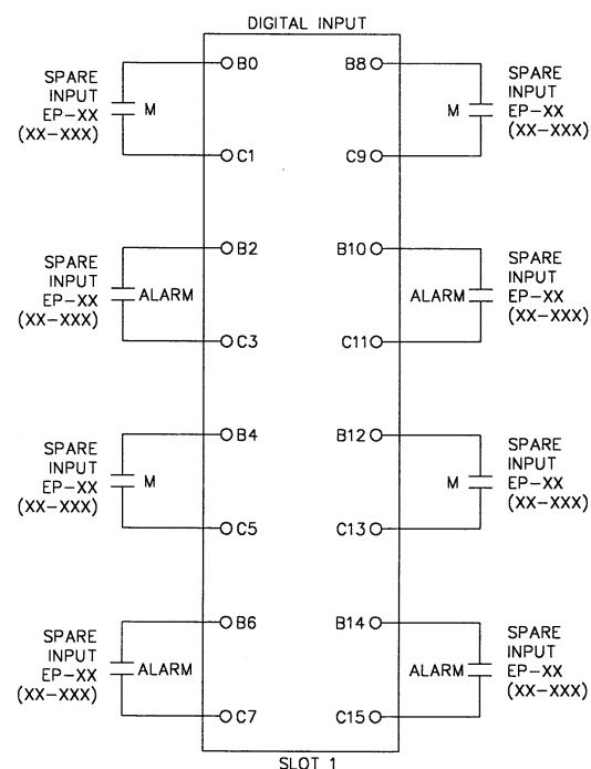
NODE 9: TRANSFORMER "A" - ADMIN. BLDG.
