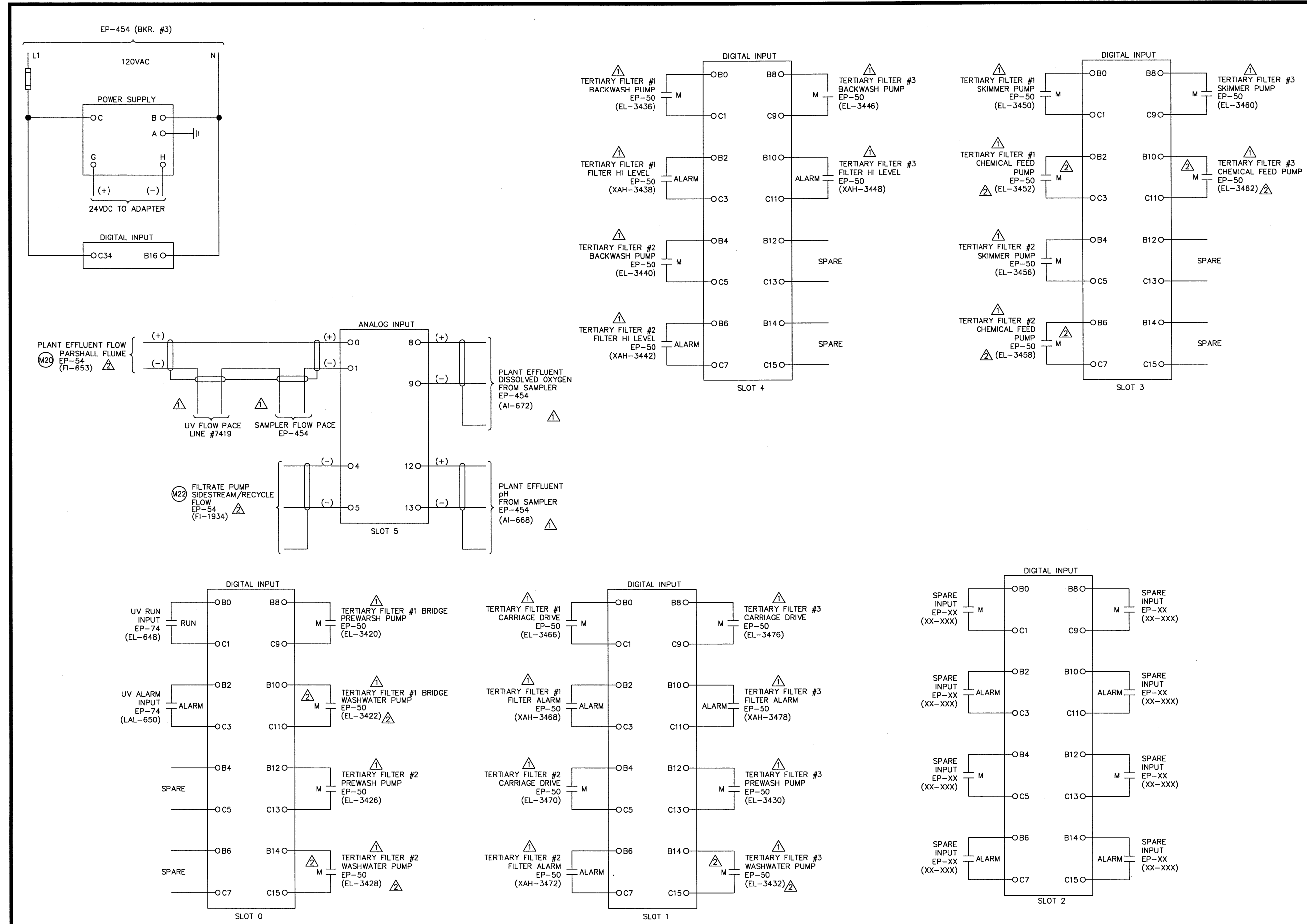
NODE 11: TRANSFORMER "D1" - TERTIARY FILTER & UV
