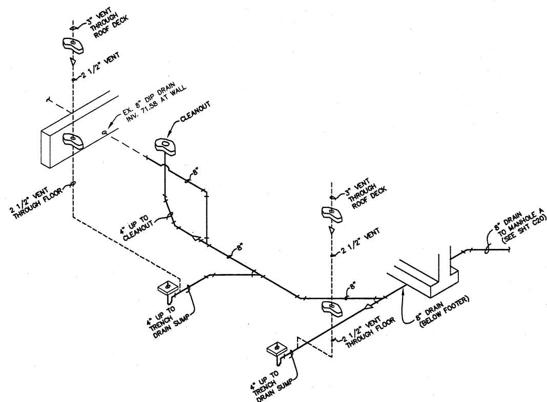
SANITARY SCHEMATIC SCALE: NONE
