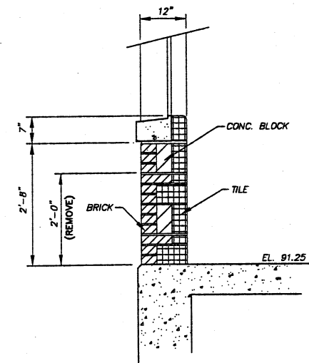
SECTION-DEMOLITION (A) M1 SCALE: 3/4" = 1'-0"
