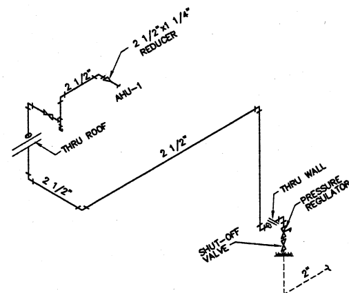
GAS SCHEMATIC
