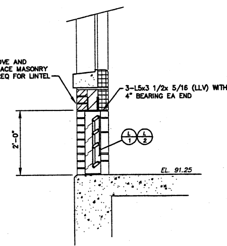
SECTION-PROPOSED (A) M1 SCALE: 3/4" = 1'-0"
