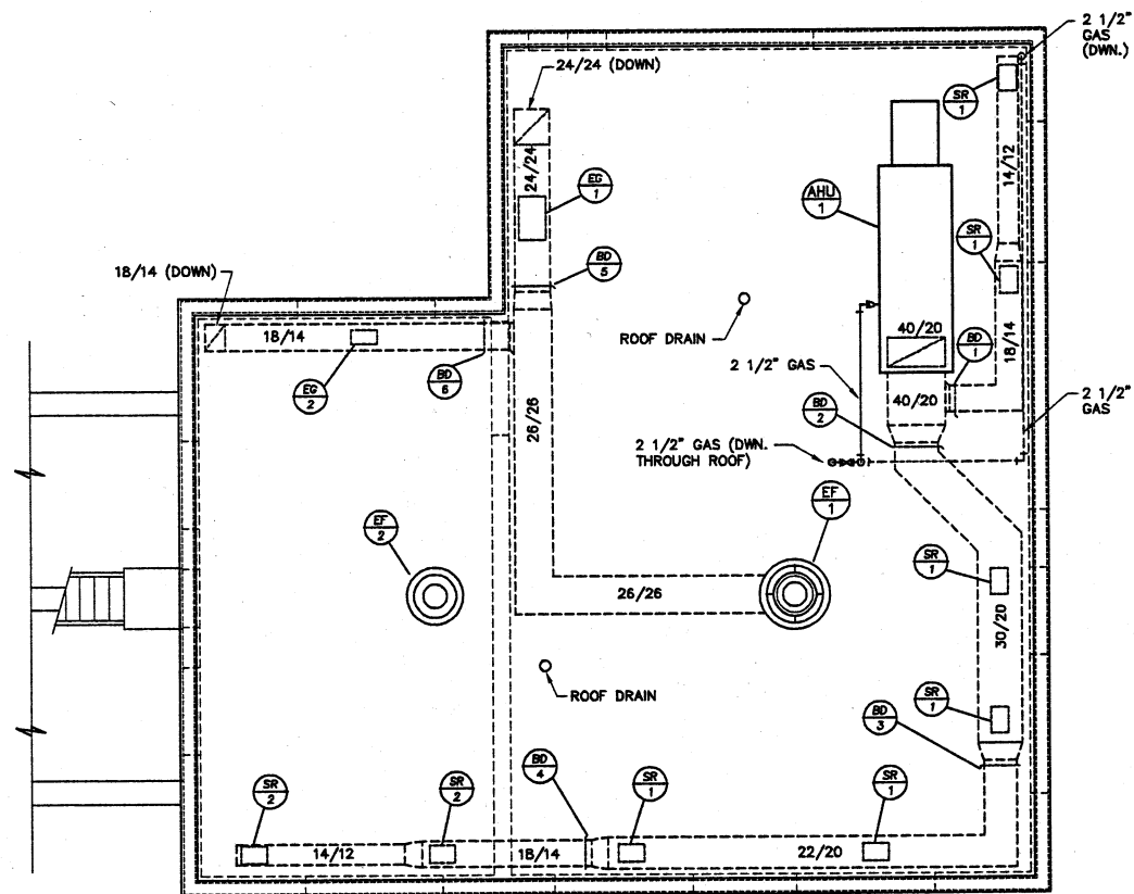
PROPOSED ROOF PLAN SCALE: 3/16" = 1'
