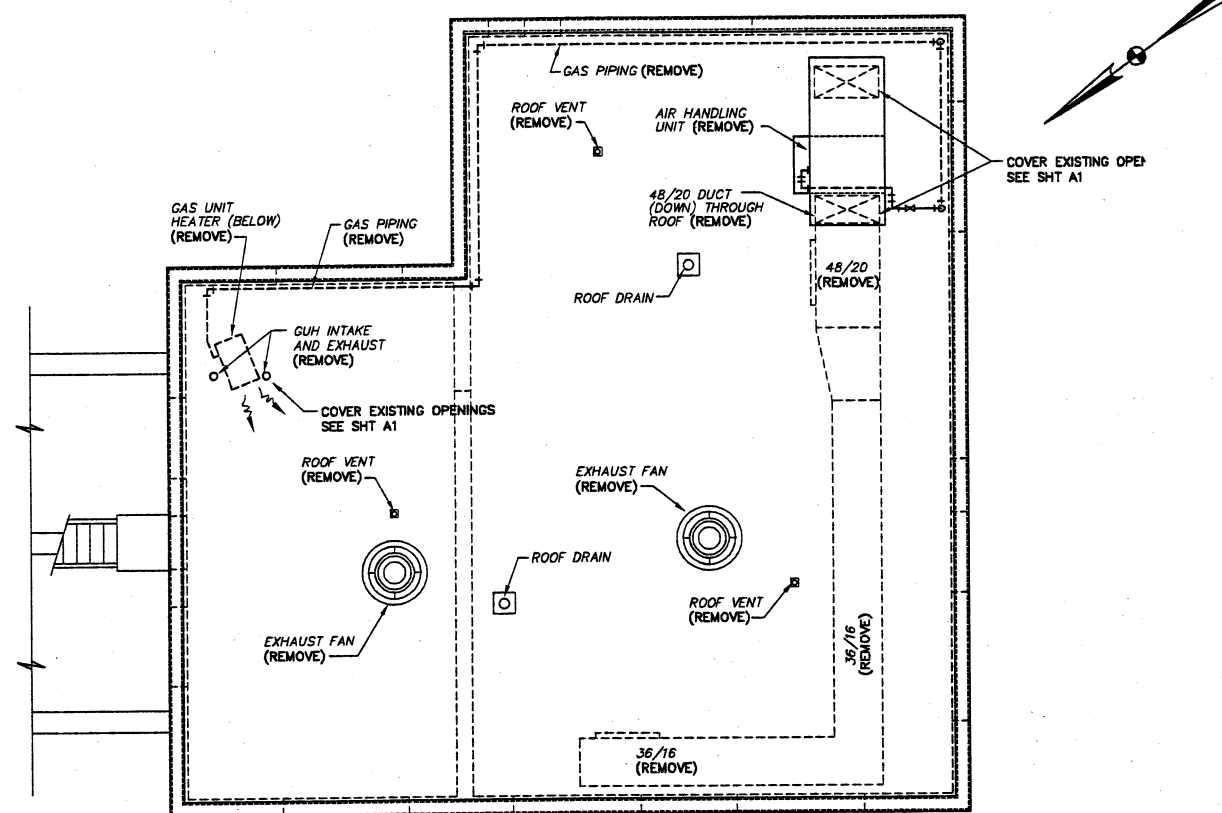
EXISTING ROOF PLAN SCALE: 3/16" = 1'
