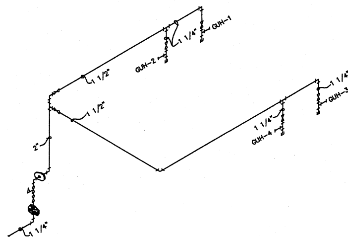
GAS SCHEMATIC SCALE: NONE
