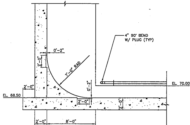
FILLET DETAIL SCALE: 1/4\"/>
