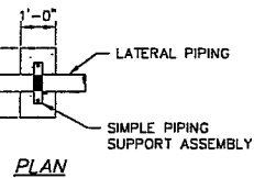
TYPE 2 CONCRETE PEDESTAL SUPPORT DETAIL
