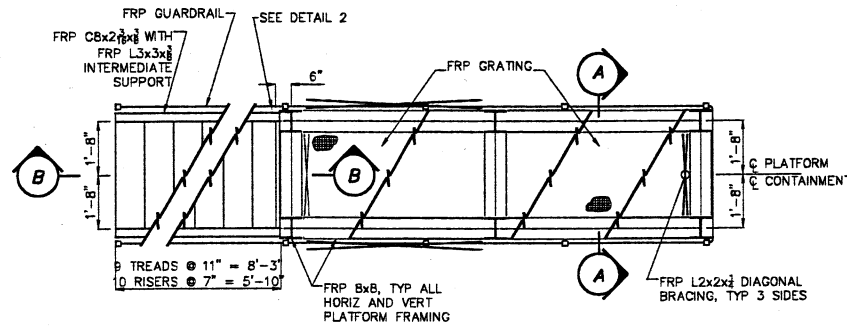
PLATFORM B @ BFP'S SCALE: 3/8" = 1'-0"
