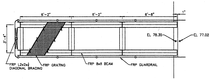
PLATFORM A @ GTB'S SCALE: 3/8" = 1'-0"
