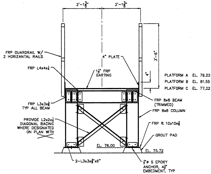
TYPICAL PLATFORM SECTION A SCALE: 3/4" = 1'-0"
