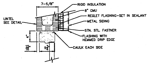
HEAD
