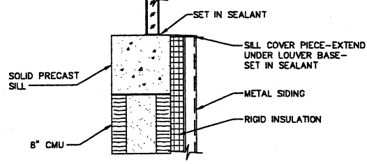
SILL
