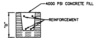
MASONRY LINTEL DETAIL
