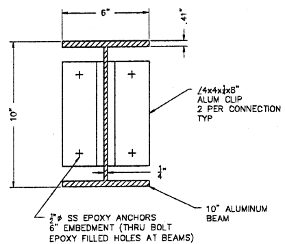
GRATING SUPPORT BEAM END CONNECTION DETAIL SCALE: 3" = 1'-0"
