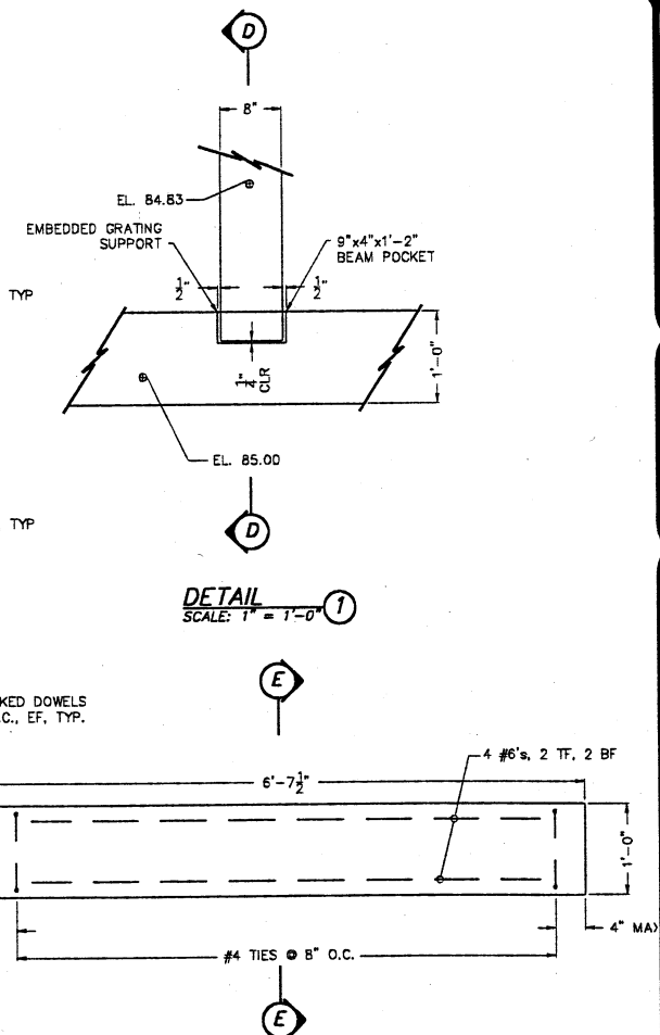
PRECAST BEAM 3 REQUIRED SCALE: 1" = 1'-0"
