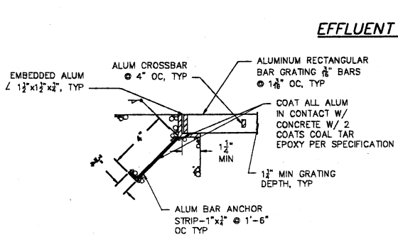
EMBEDDED GRATING SUPPORT DETAIL SCALE: 3" = 1'-0"
